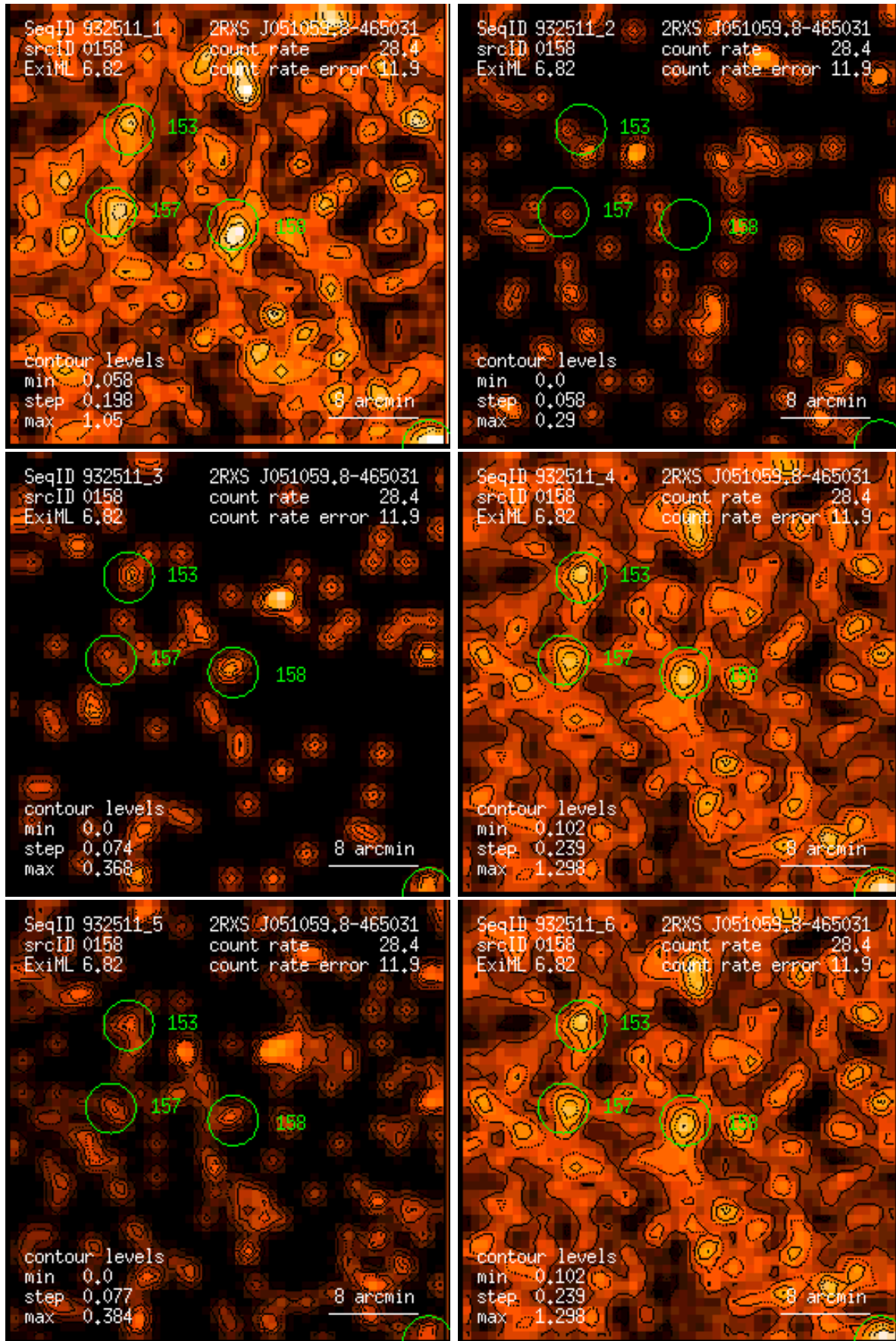
Figure 158: RASS 932511: detection 0158: band rate images, Gaussian filter: (1) PSPC channels 11 – 41, (2) 52 – 90, (3) 91 – 201, (4) 11 – 235, (5) 52 – 201, (6) 11 – 201. Broad band rates in counts/ks. Band rate contour levels in counts/ks/arcmin 2 .
