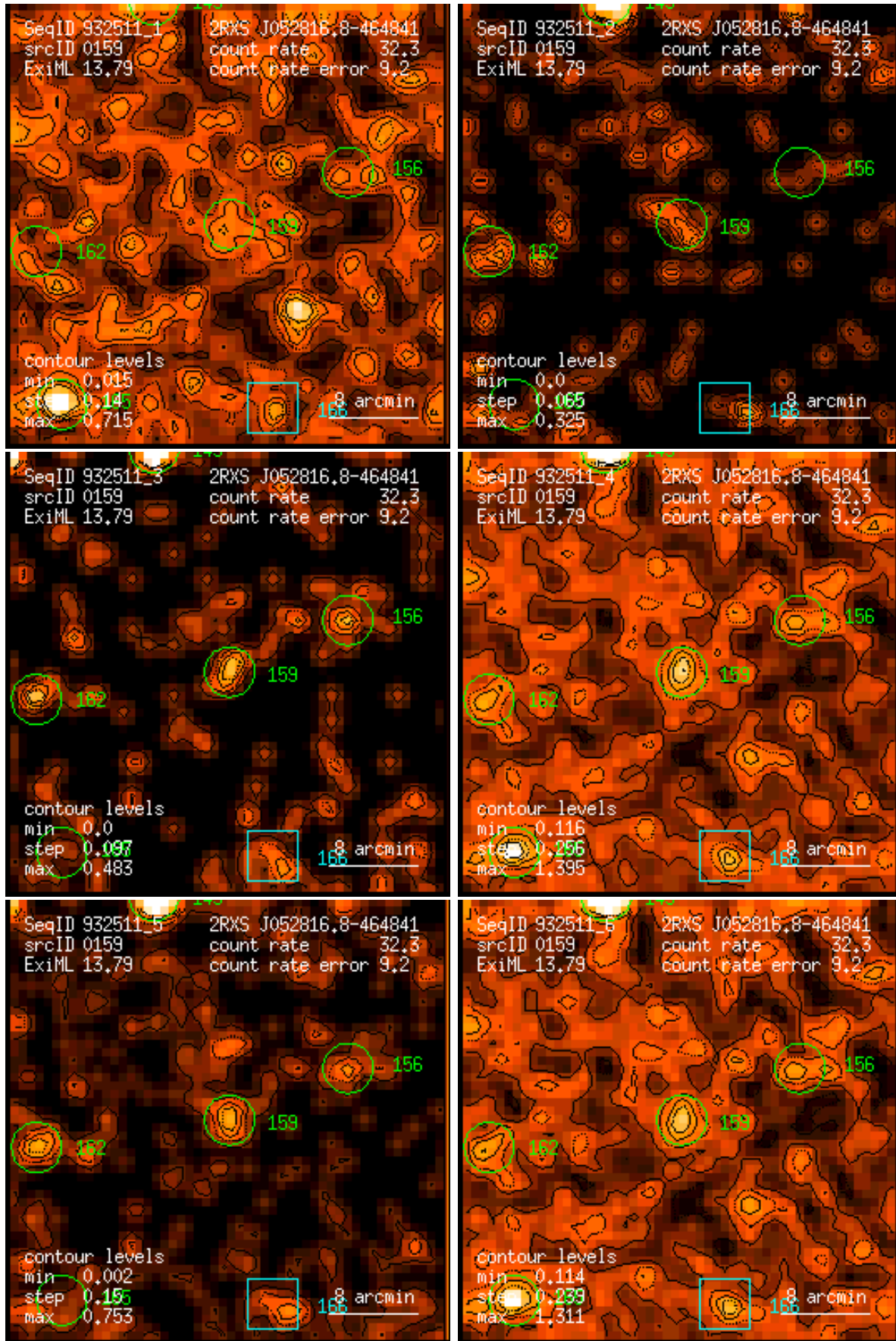
Figure 159: RASS 932511: detection 0159: band rate images, Gaussian filter: (1) PSPC channels 11 – 41, (2) 52 – 90, (3) 91 – 201, (4) 11 – 235, (5) 52 – 201, (6) 11 – 201. Broad band rates in counts/ks. Band rate contour levels in counts/ks/arcmin 2 .
