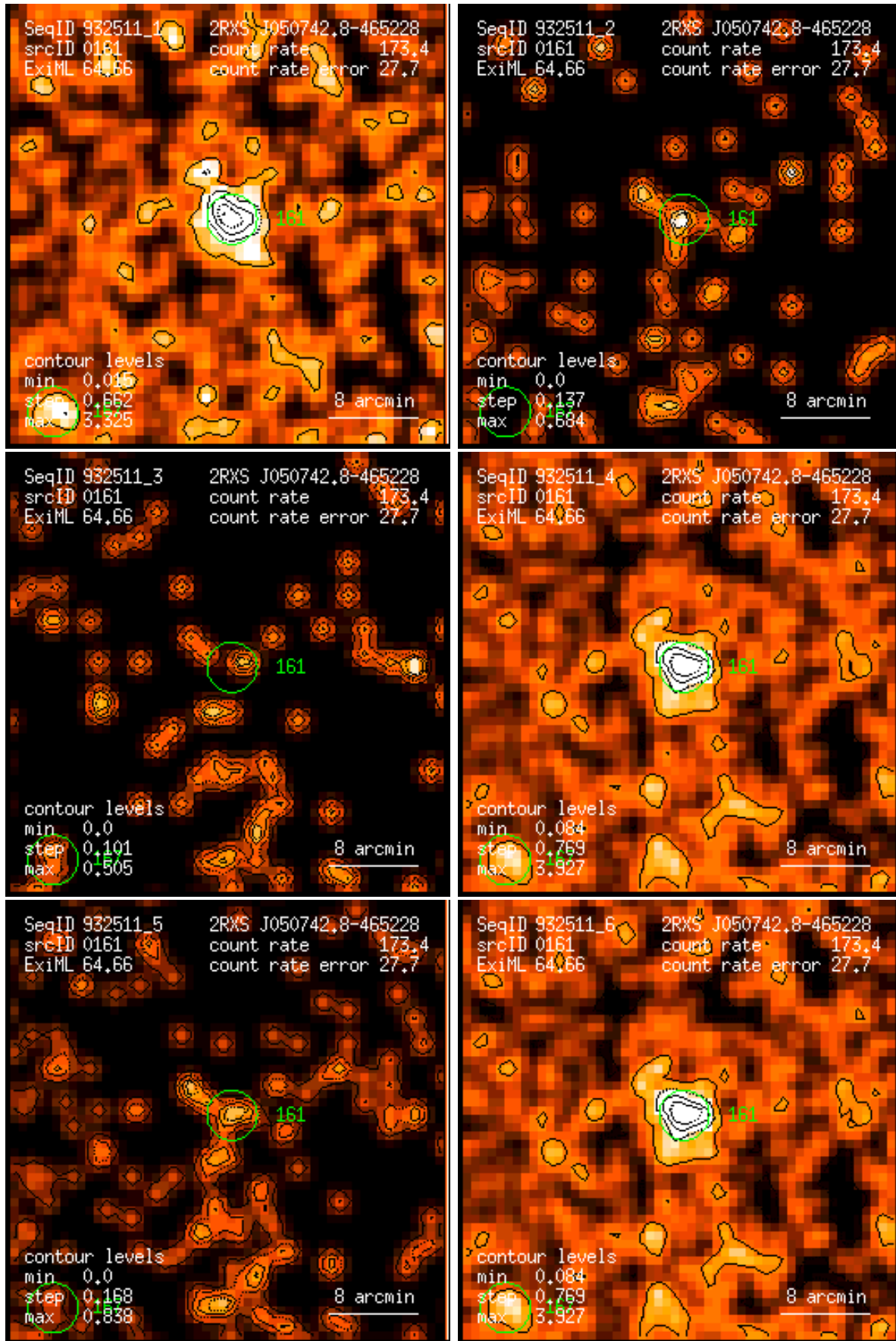
Figure 161: RASS 932511: detection 0161: band rate images, Gaussian filter: (1) PSPC channels 11 – 41, (2) 52 – 90, (3) 91 – 201, (4) 11 – 235, (5) 52 – 201, (6) 11 – 201. Broad band rates in counts/ks. Band rate contour levels in counts/ks/arcmin 2 .
