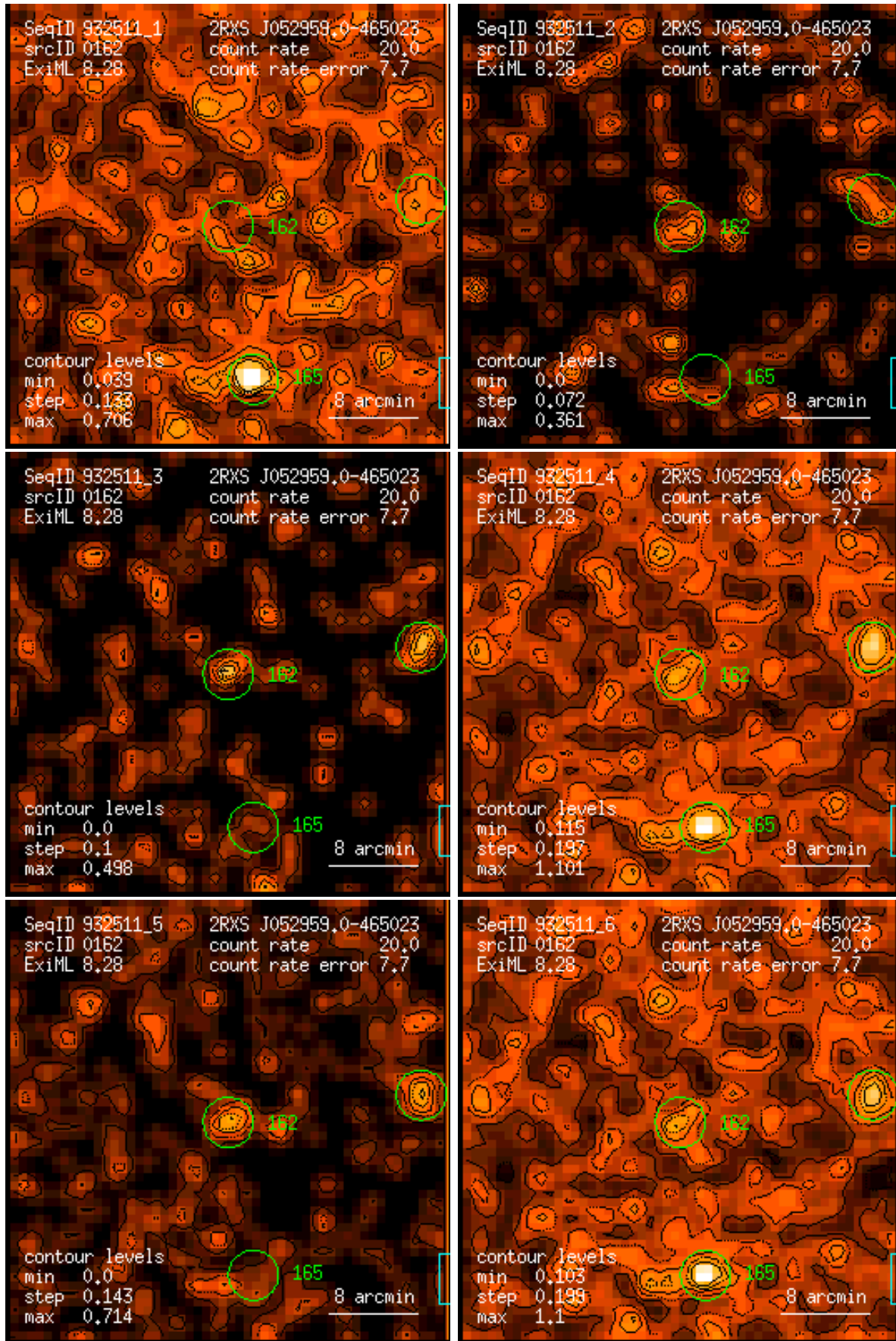
Figure 162: RASS 932511: detection 0162: band rate images, Gaussian filter: (1) PSPC channels 11 – 41, (2) 52 – 90, (3) 91 – 201, (4) 11 – 235, (5) 52 – 201, (6) 11 – 201. Broad band rates in counts/ks. Band rate contour levels in counts/ks/arcmin 2 .
