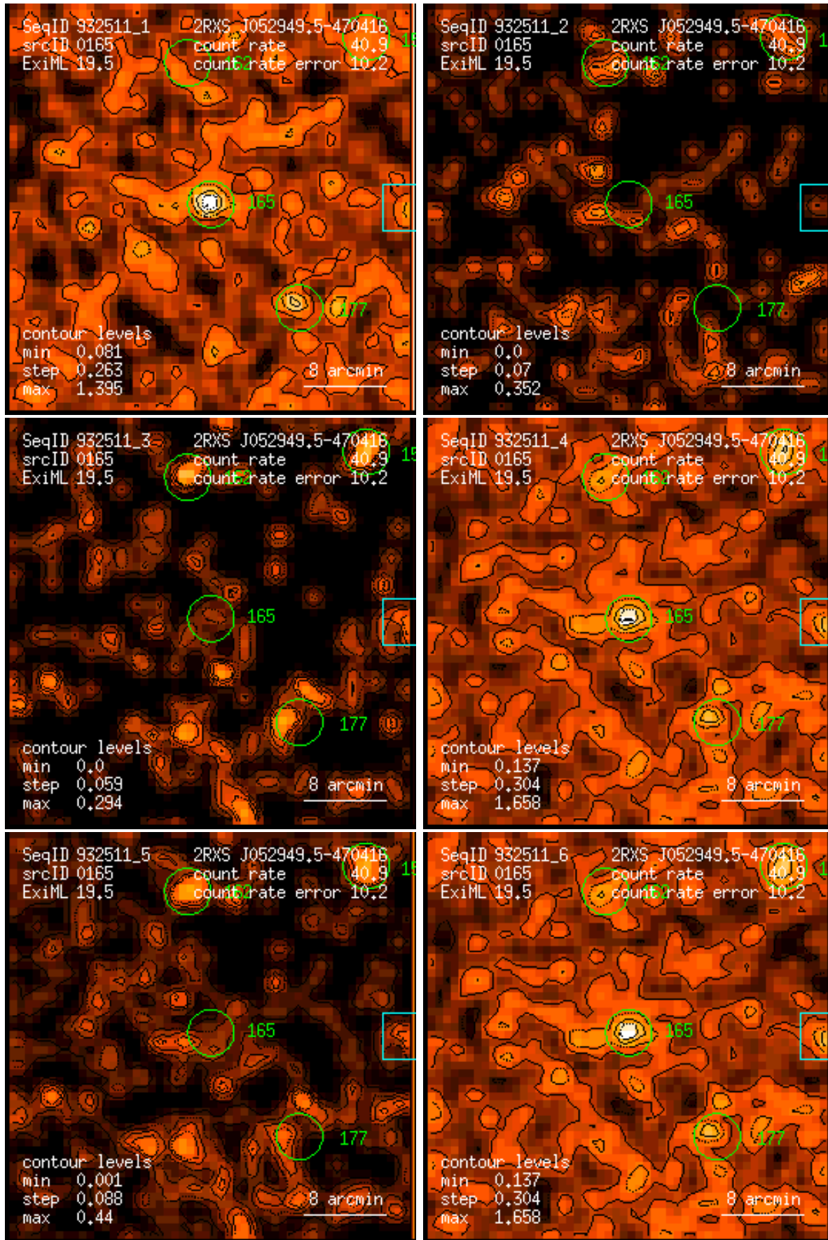
Figure 165: RASS 932511: detection 0165: band rate images, Gaussian filter: (1) PSPC channels 11 – 41, (2) 52 – 90, (3) 91 – 201, (4) 11 – 235, (5) 52 – 201, (6) 11 – 201. Broad band rates in counts/ks. Band rate contour levels in counts/ks/arcmin 2 .
