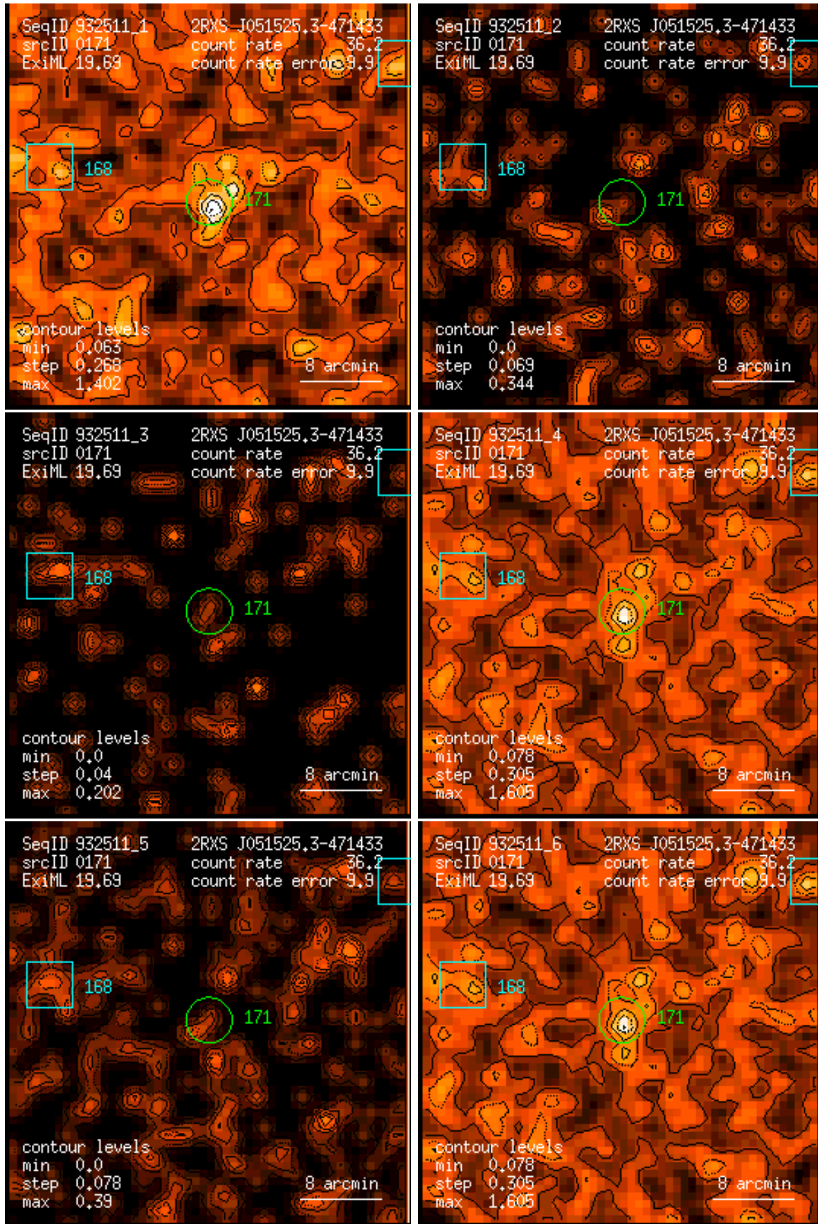
Figure 171: RASS 932511: detection 0171: band rate images, Gaussian filter: (1) PSPC channels 11 – 41, (2) 52 – 90, (3) 91 – 201, (4) 11 – 235, (5) 52 – 201, (6) 11 – 201. Broad band rates in counts/ks. Band rate contour levels in counts/ks/arcmin 2 .
