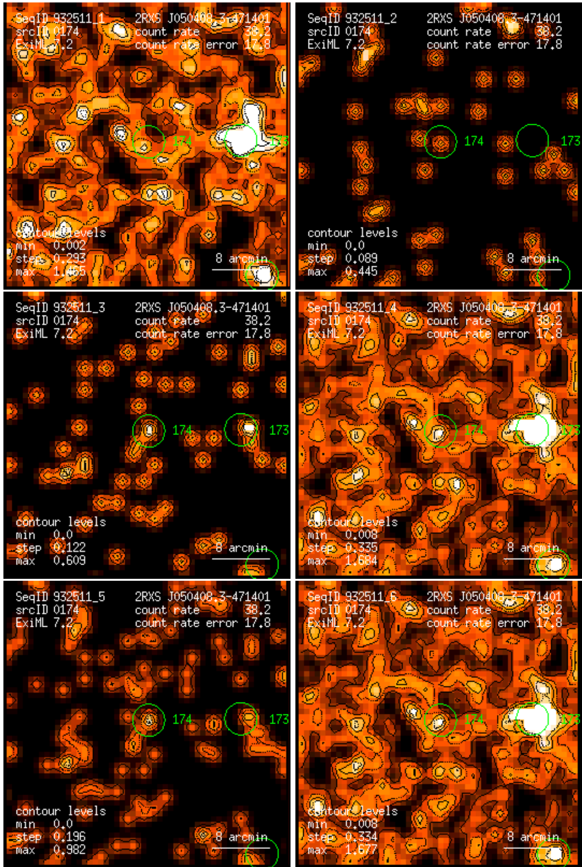
Figure 174: RASS 932511: detection 0174: band rate images, Gaussian filter: (1) PSPC channels 11 – 41, (2) 52 – 90, (3) 91 – 201, (4) 11 – 235, (5) 52 – 201, (6) 11 – 201. Broad band rates in counts/ks. Band rate contour levels in counts/ks/arcmin 2 .
