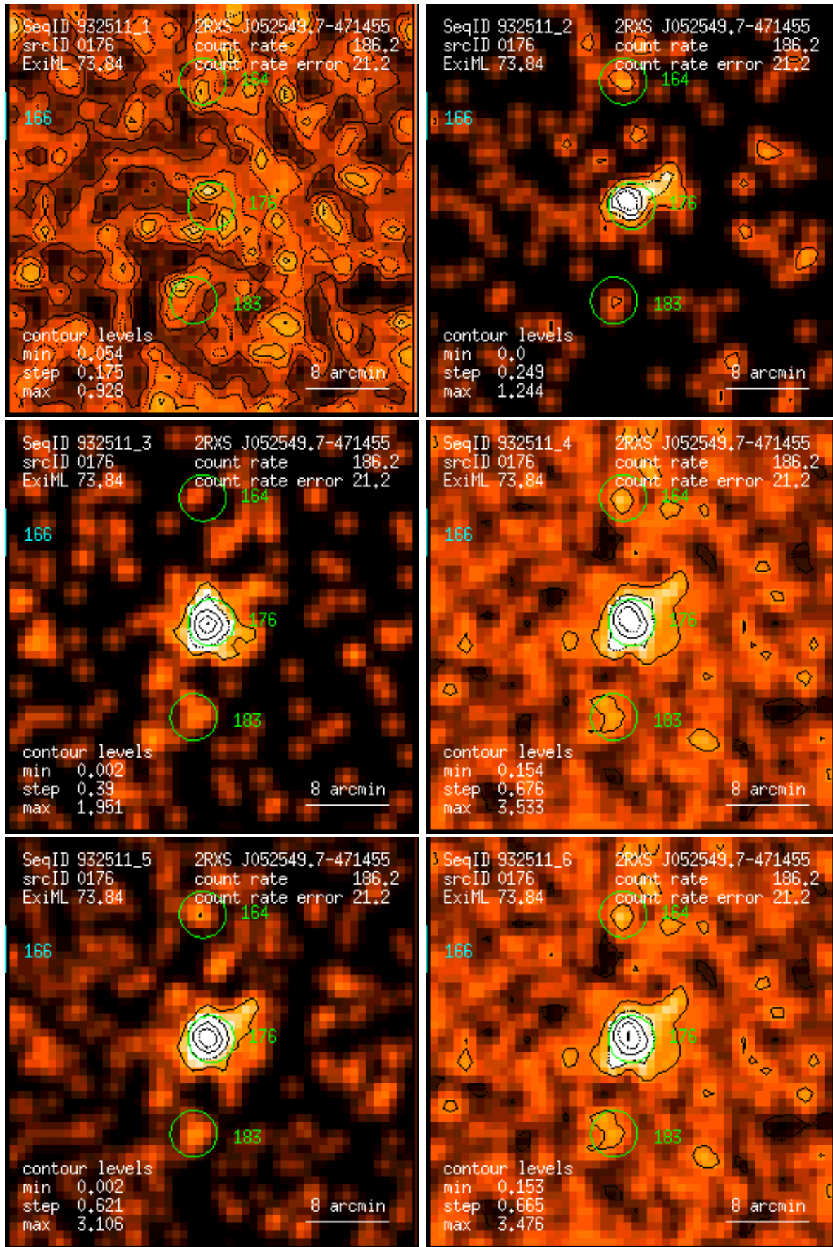
Figure 176: RASS 932511: detection 0176: band rate images, Gaussian filter: (1) PSPC channels 11 – 41, (2) 52 – 90, (3) 91 – 201, (4) 11 – 235, (5) 52 – 201, (6) 11 – 201. Broad band rates in counts/ks. Band rate contour levels in counts/ks/arcmin 2 .
