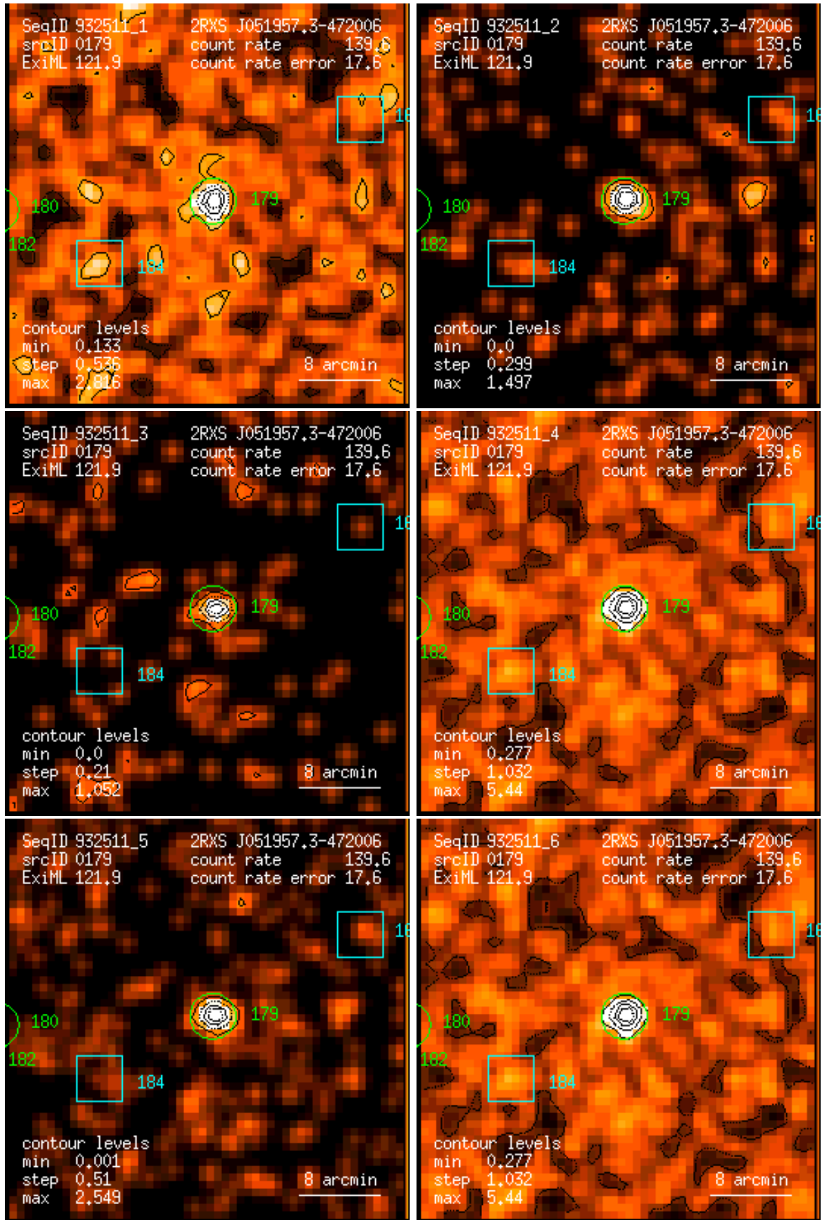
Figure 179: RASS 932511: detection 0179: band rate images, Gaussian filter: (1) PSPC channels 11 – 41, (2) 52 – 90, (3) 91 – 201, (4) 11 – 235, (5) 52 – 201, (6) 11 – 201. Broad band rates in counts/ks. Band rate contour levels in counts/ks/arcmin 2 .
