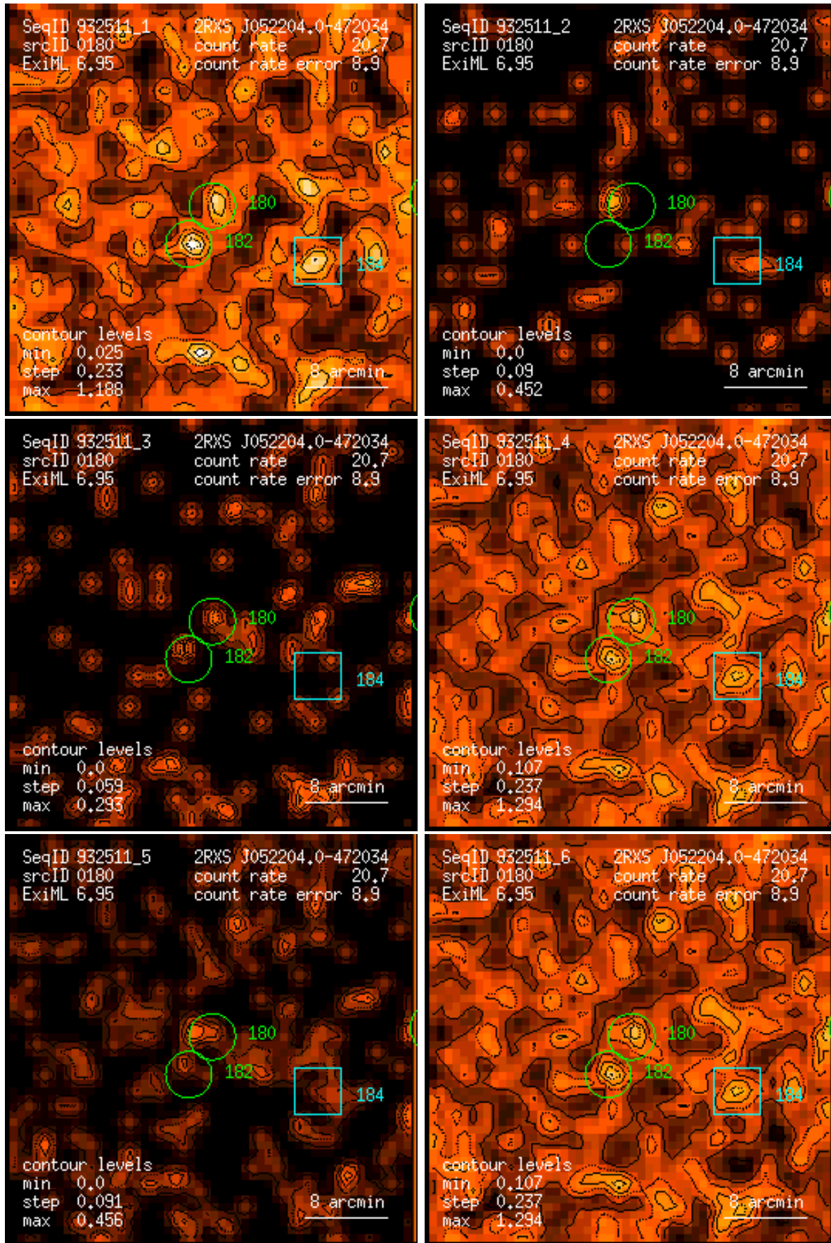
Figure 180: RASS 932511: detection 0180: band rate images, Gaussian filter: (1) PSPC channels 11 – 41, (2) 52 – 90, (3) 91 – 201, (4) 11 – 235, (5) 52 – 201, (6) 11 – 201. Broad band rates in counts/ks. Band rate contour levels in counts/ks/arcmin 2 .
