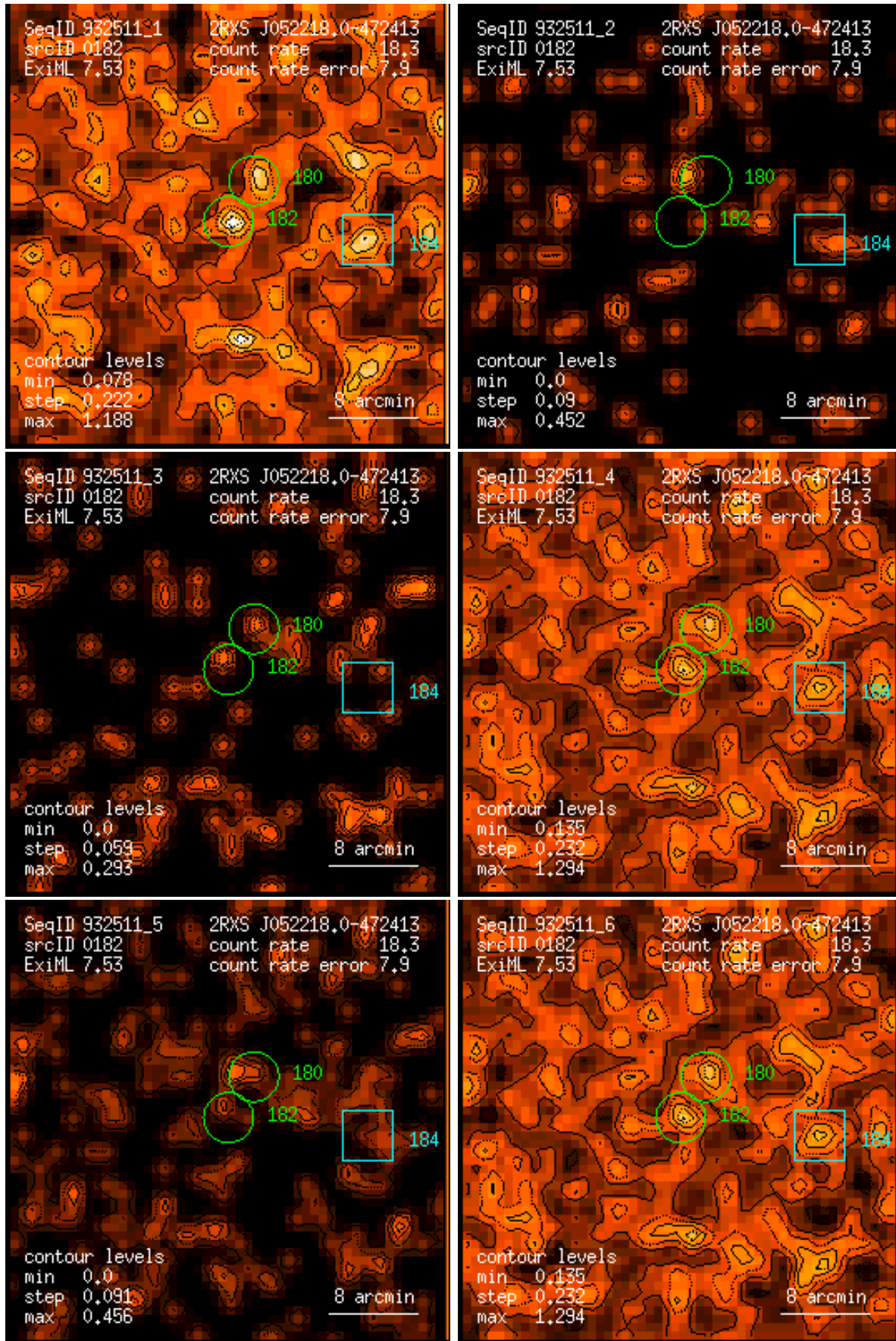
Figure 182: RASS 932511: detection 0182: band rate images, Gaussian filter: (1) PSPC channels 11 – 41, (2) 52 – 90, (3) 91 – 201, (4) 11 – 235, (5) 52 – 201, (6) 11 – 201. Broad band rates in counts/ks. Band rate contour levels in counts/ks/arcmin 2 .
