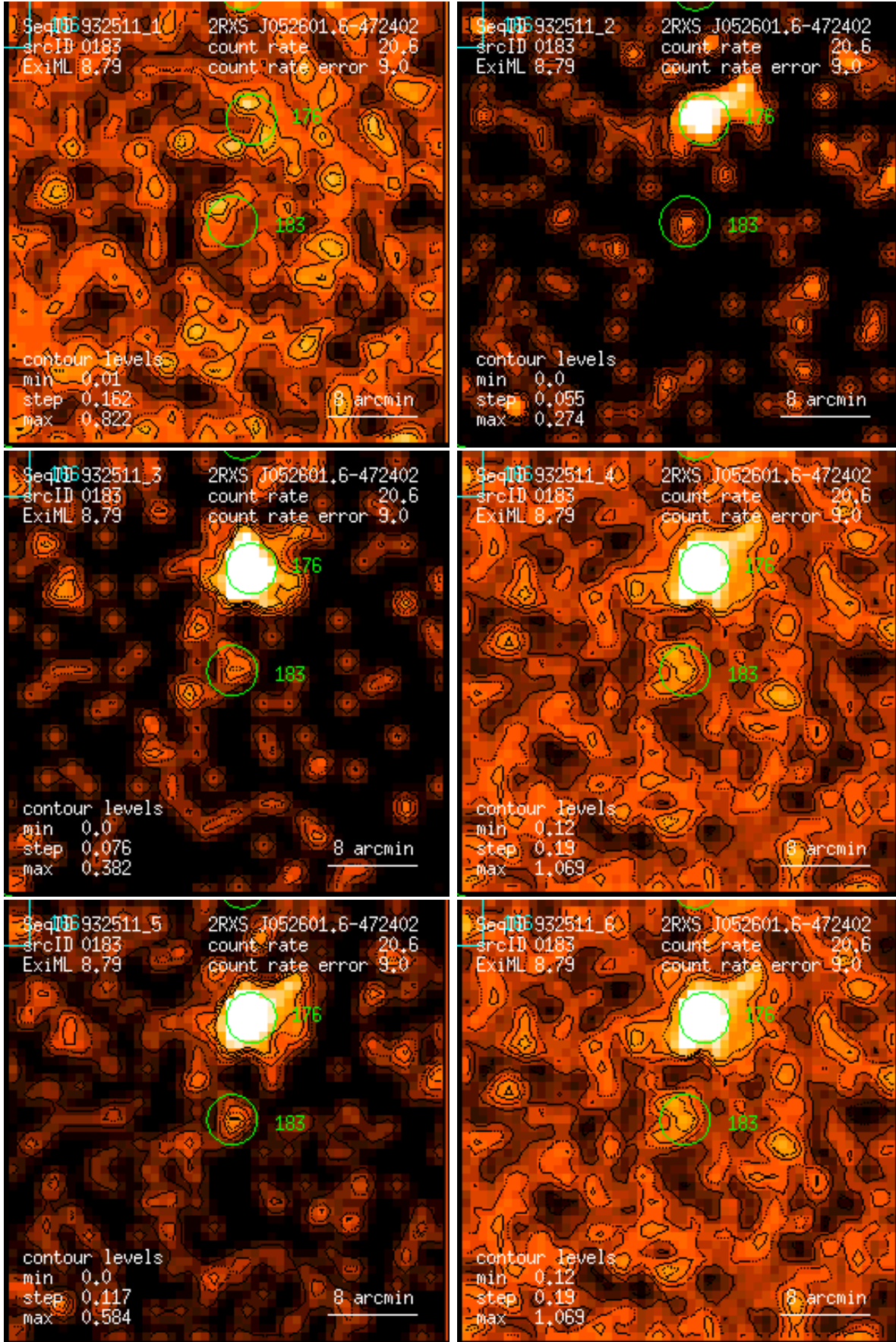
Figure 183: RASS 932511: detection 0183: band rate images, Gaussian filter: (1) PSPC channels 11 – 41, (2) 52 – 90, (3) 91 – 201, (4) 11 – 235, (5) 52 – 201, (6) 11 – 201. Broad band rates in counts/ks. Band rate contour levels in counts/ks/arcmin 2 .
