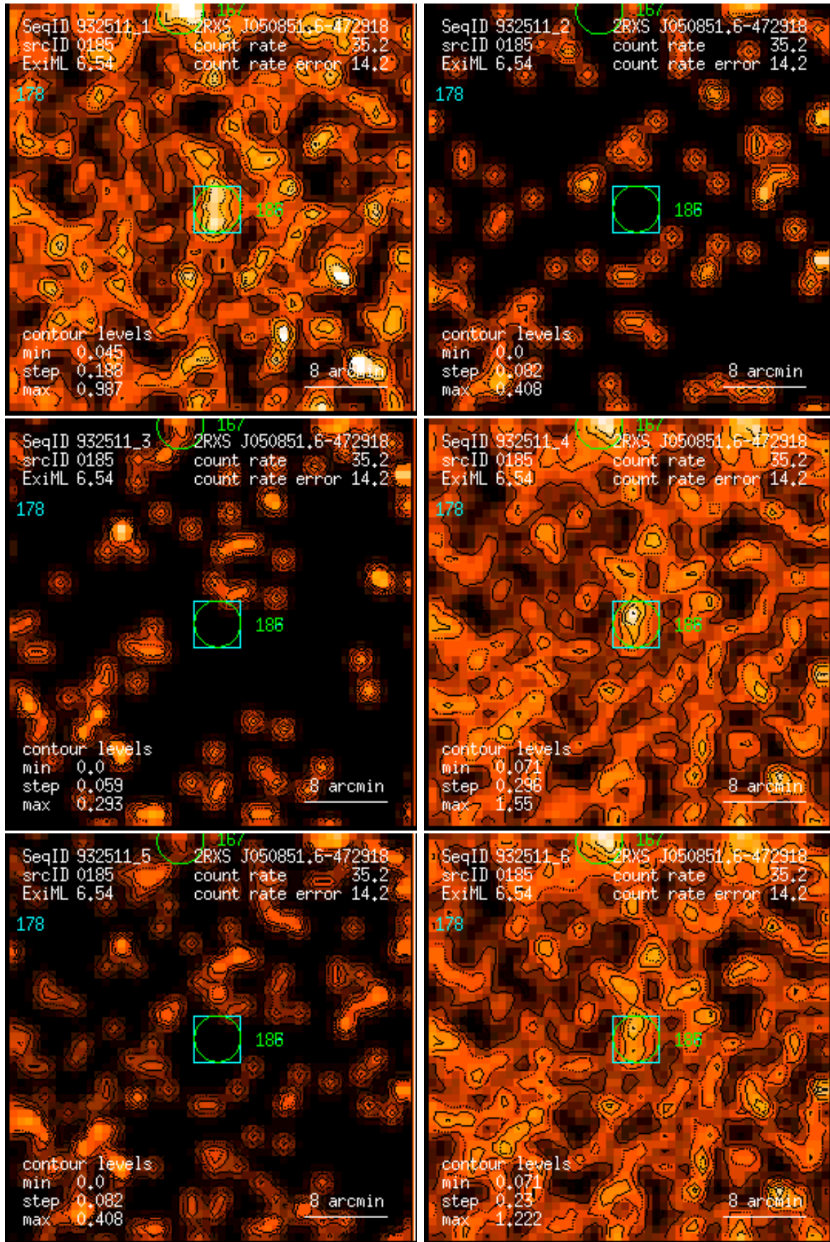
Figure 185: RASS 932511: detection 0185: band rate images, Gaussian filter: (1) PSPC channels 11 – 41, (2) 52 – 90, (3) 91 – 201, (4) 11 – 235, (5) 52 – 201, (6) 11 – 201. Broad band rates in counts/ks. Band rate contour levels in counts/ks/arcmin 2 .
