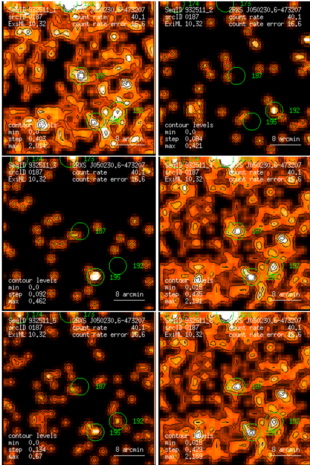
Figure 187: RASS 932511: detection 0187: band rate images, Gaussian filter: (1) PSPC channels 11 – 41, (2) 52 – 90, (3) 91 – 201, (4) 11 – 235, (5) 52 – 201, (6) 11 – 201. Broad band rates in counts/ks. Band rate contour levels in counts/ks/arcmin 2 .
