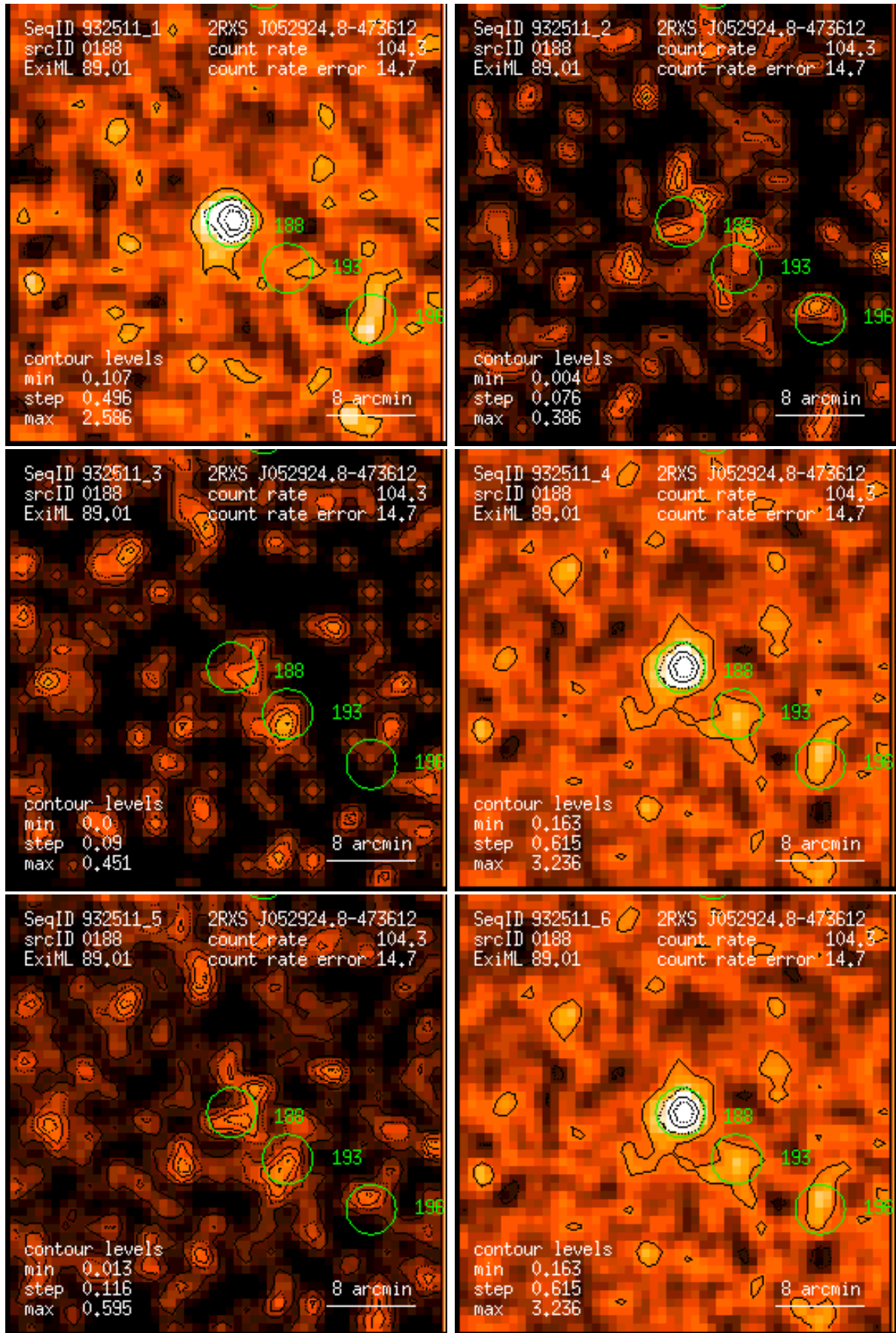
Figure 188: RASS 932511: detection 0188: band rate images, Gaussian filter: (1) PSPC channels 11 – 41, (2) 52 – 90, (3) 91 – 201, (4) 11 – 235, (5) 52 – 201, (6) 11 – 201. Broad band rates in counts/ks. Band rate contour levels in counts/ks/arcmin 2 .
