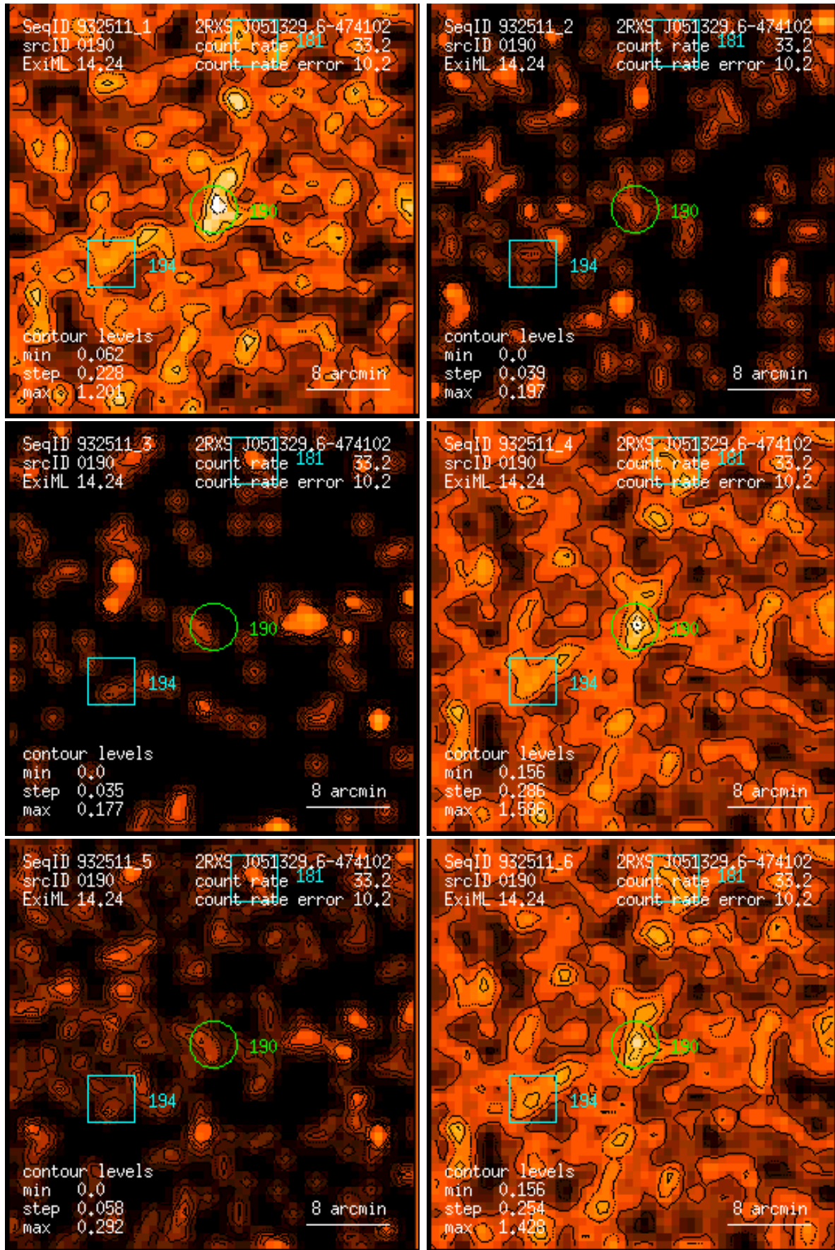
Figure 190: RASS 932511: detection 0190: band rate images, Gaussian filter: (1) PSPC channels 11 – 41, (2) 52 – 90, (3) 91 – 201, (4) 11 – 235, (5) 52 – 201, (6) 11 – 201. Broad band rates in counts/ks. Band rate contour levels in counts/ks/arcmin 2 .
