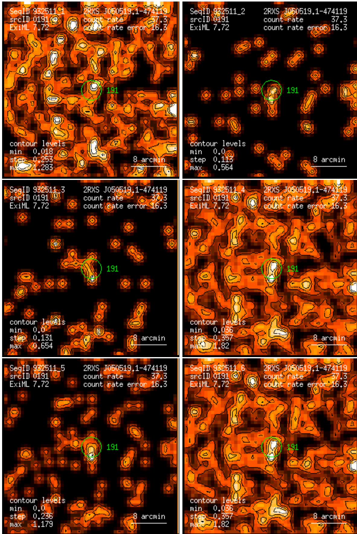
Figure 191: RASS 932511: detection 0191: band rate images, Gaussian filter: (1) PSPC channels 11 – 41, (2) 52 – 90, (3) 91 – 201, (4) 11 – 235, (5) 52 – 201, (6) 11 – 201. Broad band rates in counts/ks. Band rate contour levels in counts/ks/arcmin 2 .
