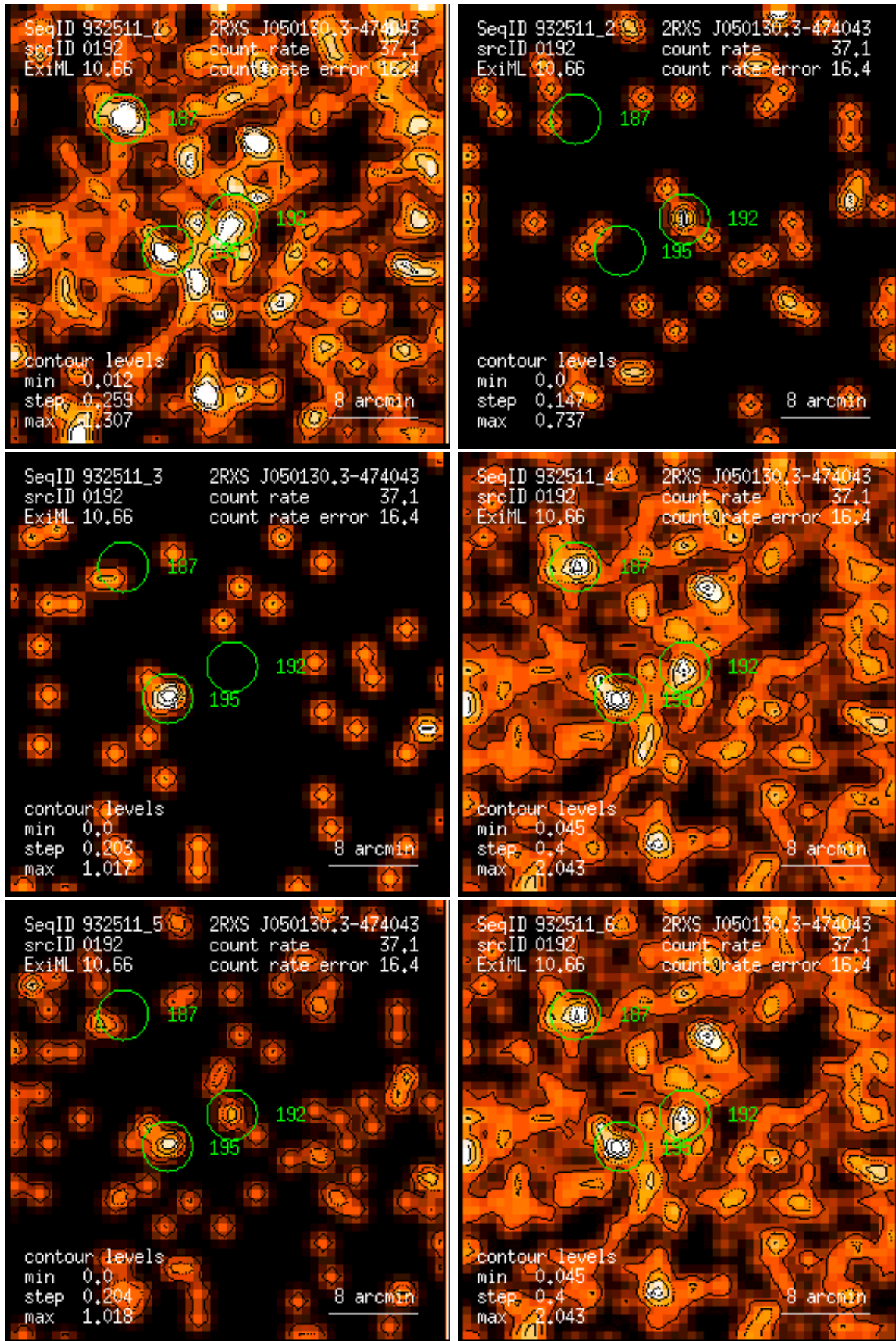
Figure 192: RASS 932511: detection 0192: band rate images, Gaussian filter: (1) PSPC channels 11 – 41, (2) 52 – 90, (3) 91 – 201, (4) 11 – 235, (5) 52 – 201, (6) 11 – 201. Broad band rates in counts/ks. Band rate contour levels in counts/ks/arcmin 2 .
