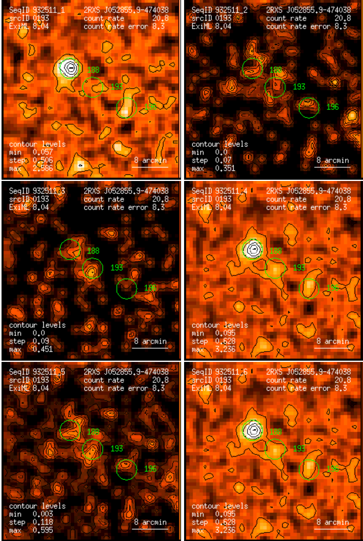
Figure 193: RASS 932511: detection 0193: band rate images, Gaussian filter: (1) PSPC channels 11 – 41, (2) 52 – 90, (3) 91 – 201, (4) 11 – 235, (5) 52 – 201, (6) 11 – 201. Broad band rates in counts/ks. Band rate contour levels in counts/ks/arcmin 2 .
