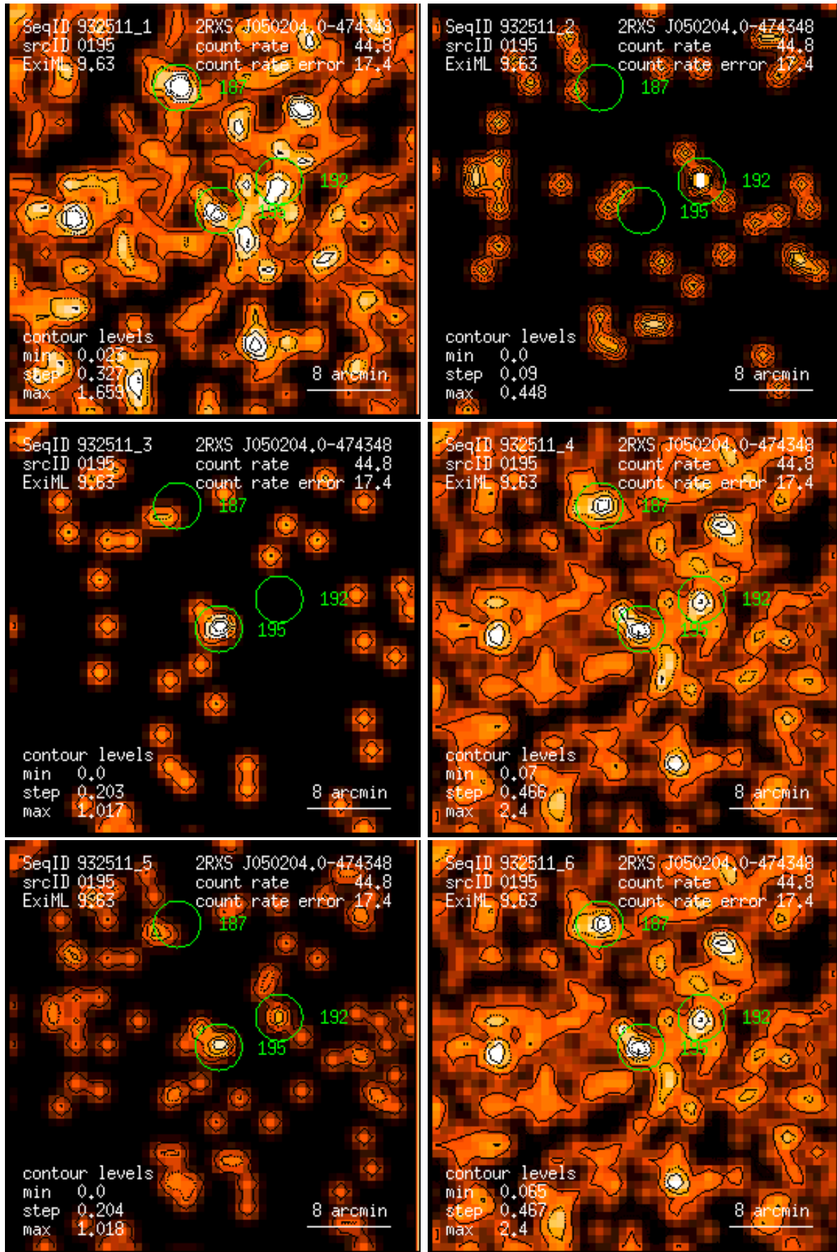
Figure 195: RASS 932511: detection 0195: band rate images, Gaussian filter: (1) PSPC channels 11 – 41, (2) 52 – 90, (3) 91 – 201, (4) 11 – 235, (5) 52 – 201, (6) 11 – 201. Broad band rates in counts/ks. Band rate contour levels in counts/ks/arcmin 2 .
