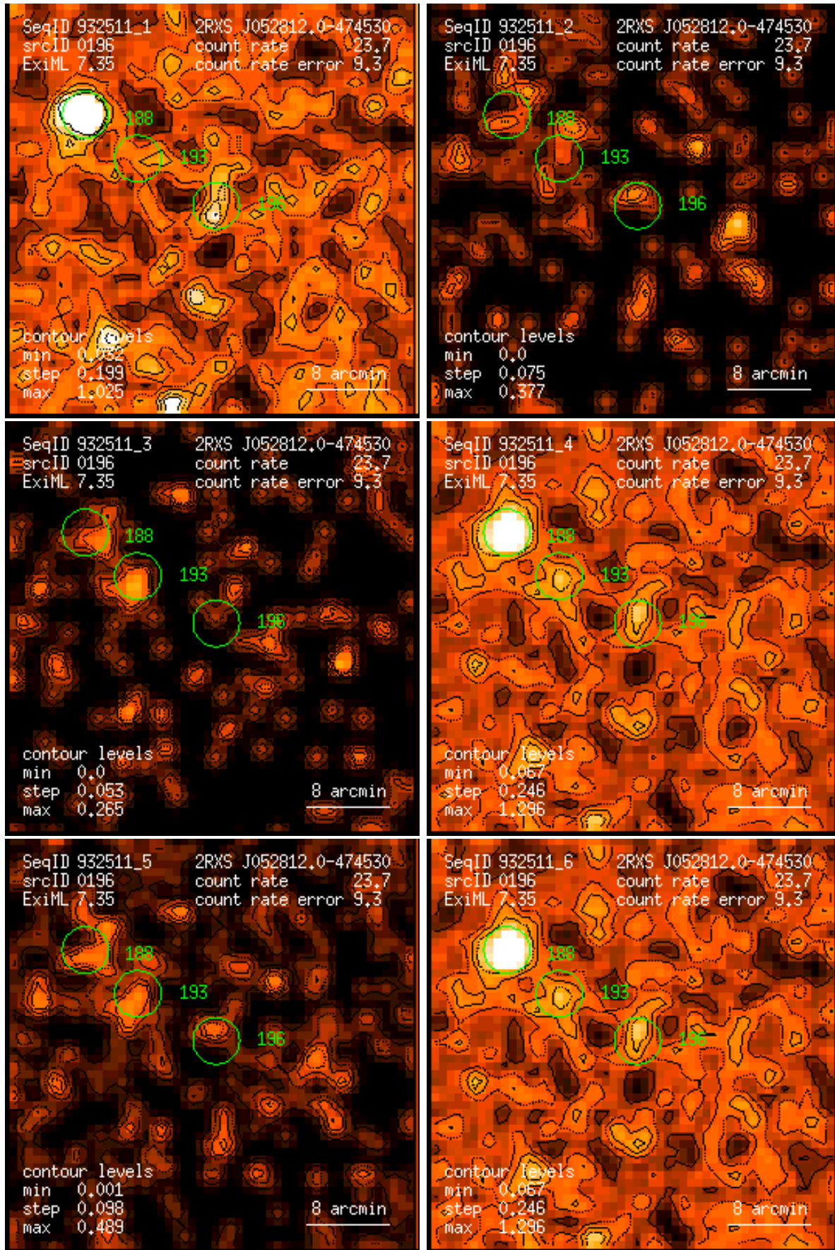
Figure 196: RASS 932511: detection 0196: band rate images, Gaussian filter: (1) PSPC channels 11 – 41, (2) 52 – 90, (3) 91 – 201, (4) 11 – 235, (5) 52 – 201, (6) 11 – 201. Broad band rates in counts/ks. Band rate contour levels in counts/ks/arcmin 2 .
