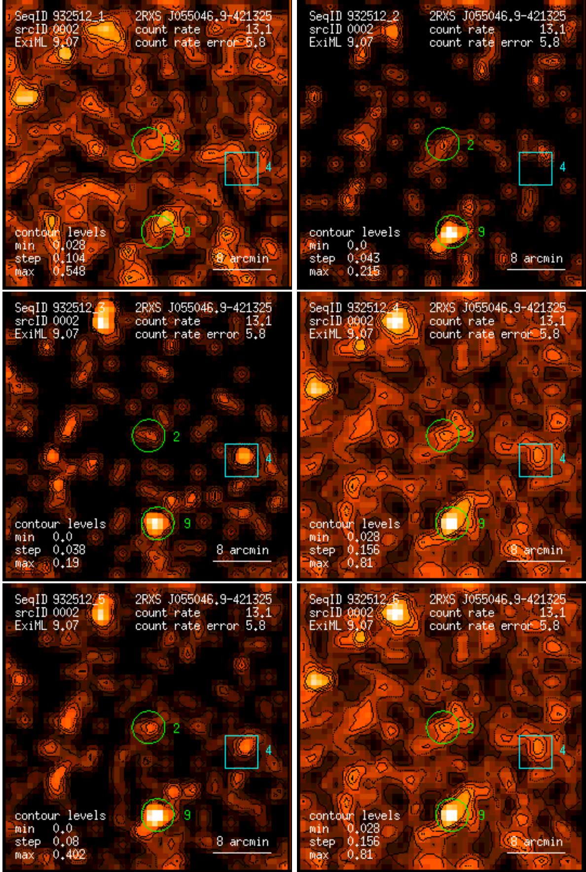
Figure 2: RASS 932512: detection 0002: band rate images, Gaussian filter: (1) PSPC channels 11 – 41, (2) 52 – 90, (3) 91 – 201, (4) 11 – 235, (5) 52 – 201, (6) 11 – 201. Broad band rates in counts/ks. Band rate contour levels in counts/ks/arcmin 2 .
