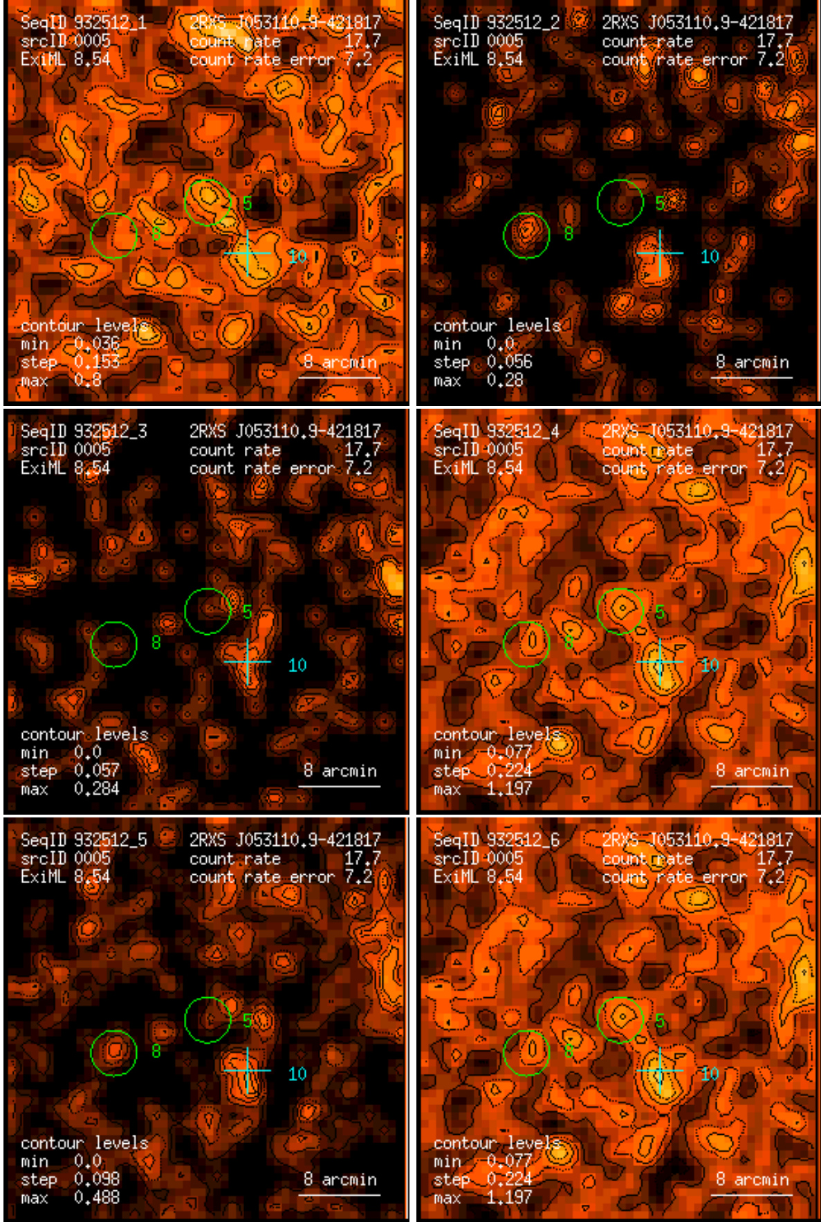
Figure 5: RASS 932512: detection 0005: band rate images, Gaussian filter: (1) PSPC channels 11 – 41, (2) 52 – 90, (3) 91 – 201, (4) 11 – 235, (5) 52 – 201, (6) 11 – 201. Broad band rates in counts/ks. Band rate contour levels in counts/ks/arcmin 2 .
