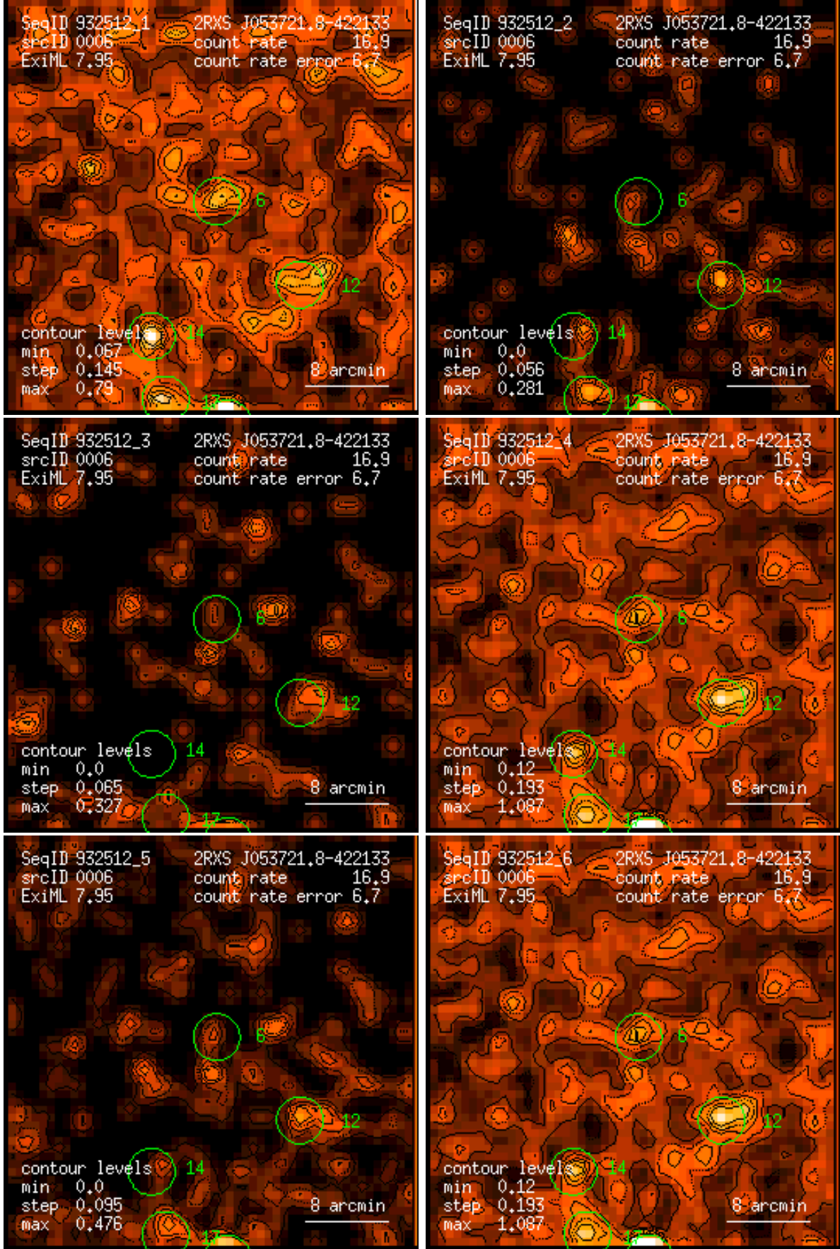
Figure 6: RASS 932512: detection 0006: band rate images, Gaussian filter: (1) PSPC channels 11 – 41, (2) 52 – 90, (3) 91 – 201, (4) 11 – 235, (5) 52 – 201, (6) 11 – 201. Broad band rates in counts/ks. Band rate contour levels in counts/ks/arcmin 2 .
