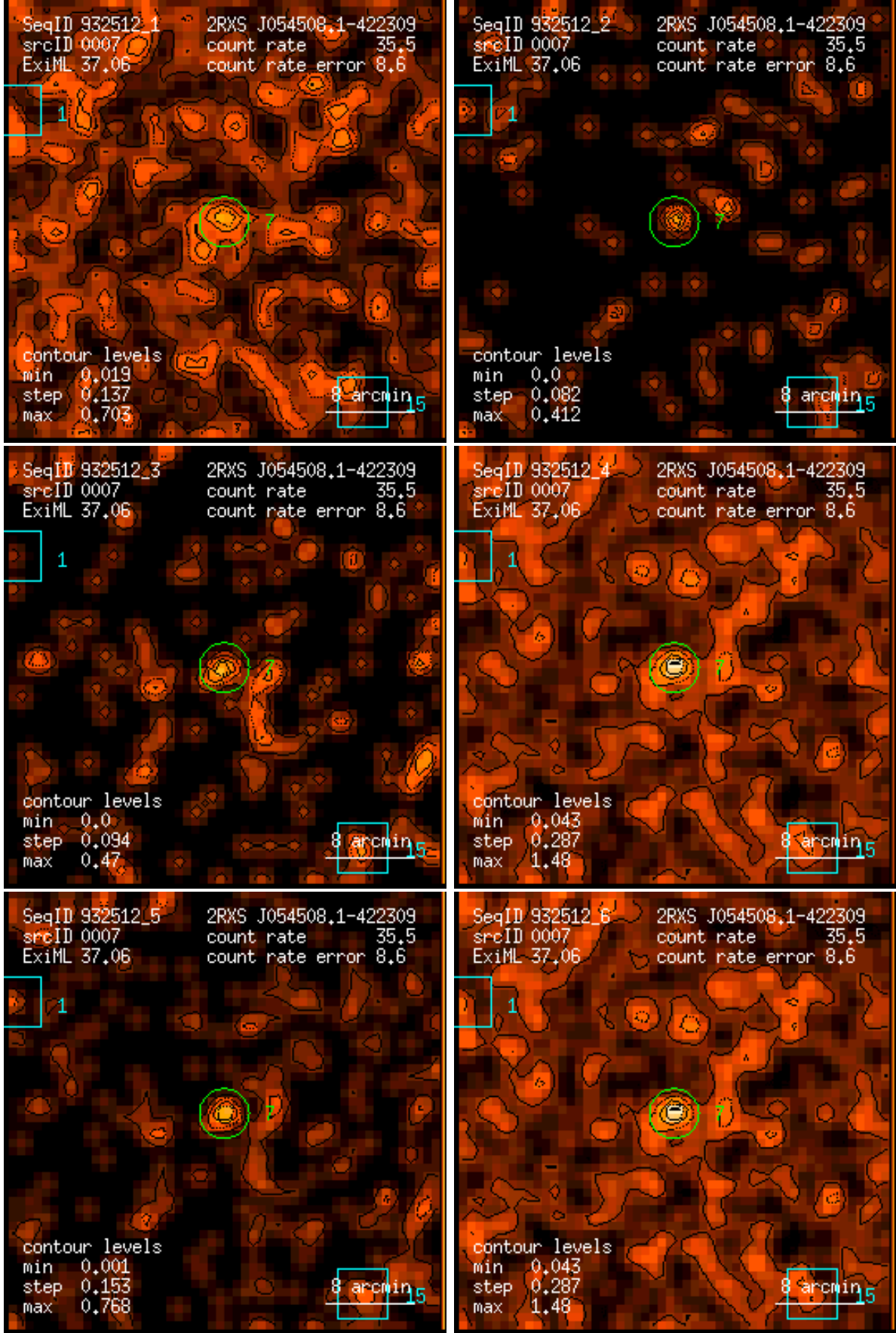
Figure 7: RASS 932512: detection 0007: band rate images, Gaussian filter: (1) PSPC channels 11 – 41, (2) 52 – 90, (3) 91 – 201, (4) 11 – 235, (5) 52 – 201, (6) 11 – 201. Broad band rates in counts/ks. Band rate contour levels in counts/ks/arcmin 2 .
