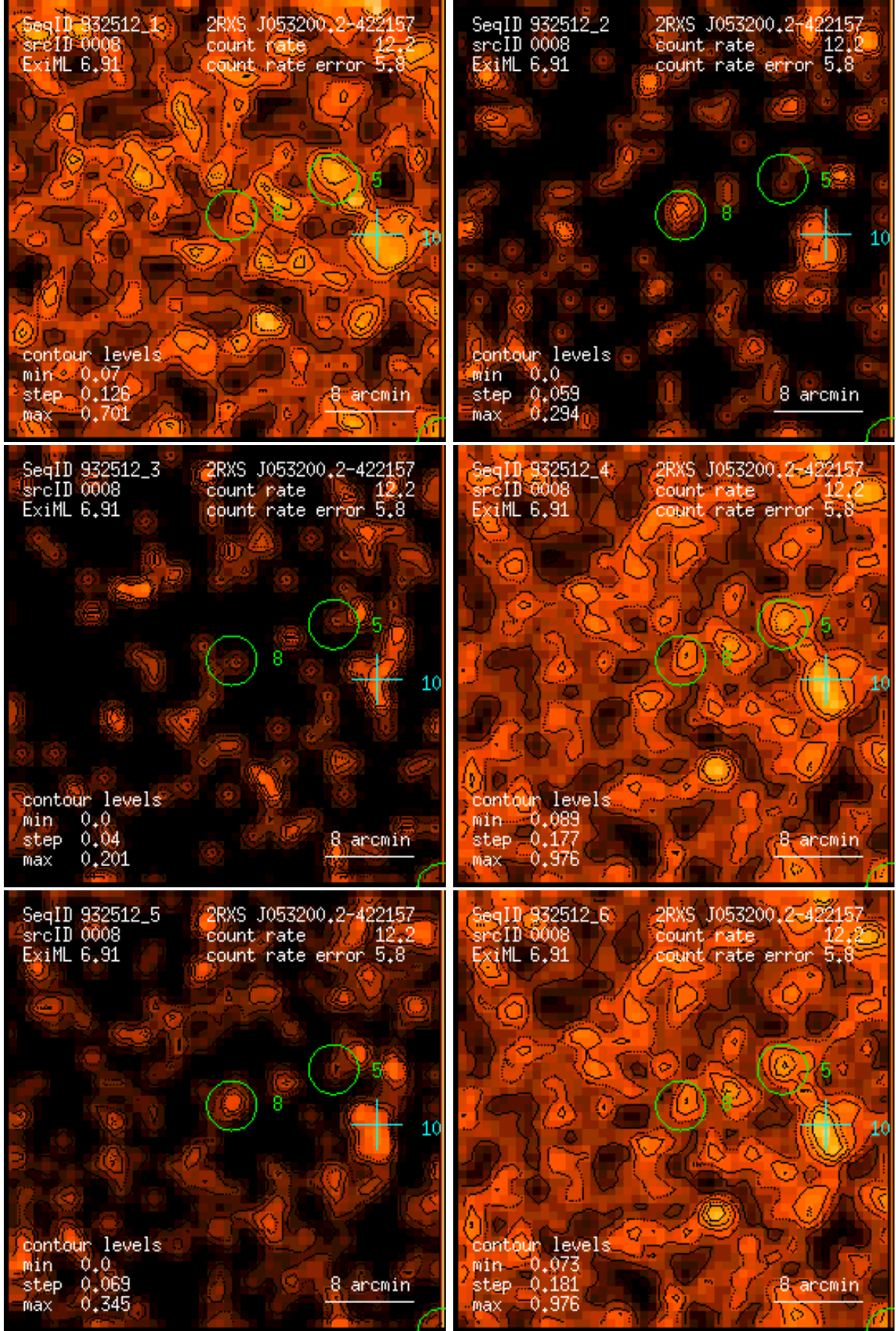
Figure 8: RASS 932512: detection 0008: band rate images, Gaussian filter: (1) PSPC channels 11 – 41, (2) 52 – 90, (3) 91 – 201, (4) 11 – 235, (5) 52 – 201, (6) 11 – 201. Broad band rates in counts/ks. Band rate contour levels in counts/ks/arcmin 2 .
