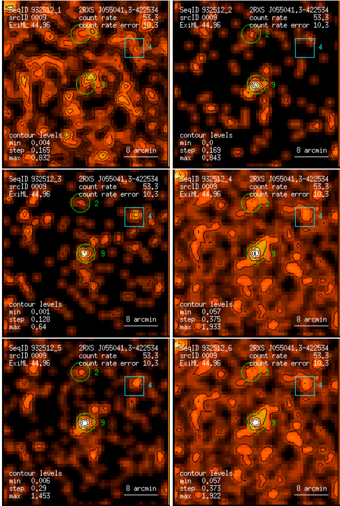
Figure 9: RASS 932512: detection 0009: band rate images, Gaussian filter: (1) PSPC channels 11 – 41, (2) 52 – 90, (3) 91 – 201, (4) 11 – 235, (5) 52 – 201, (6) 11 – 201. Broad band rates in counts/ks. Band rate contour levels in counts/ks/arcmin 2 .
