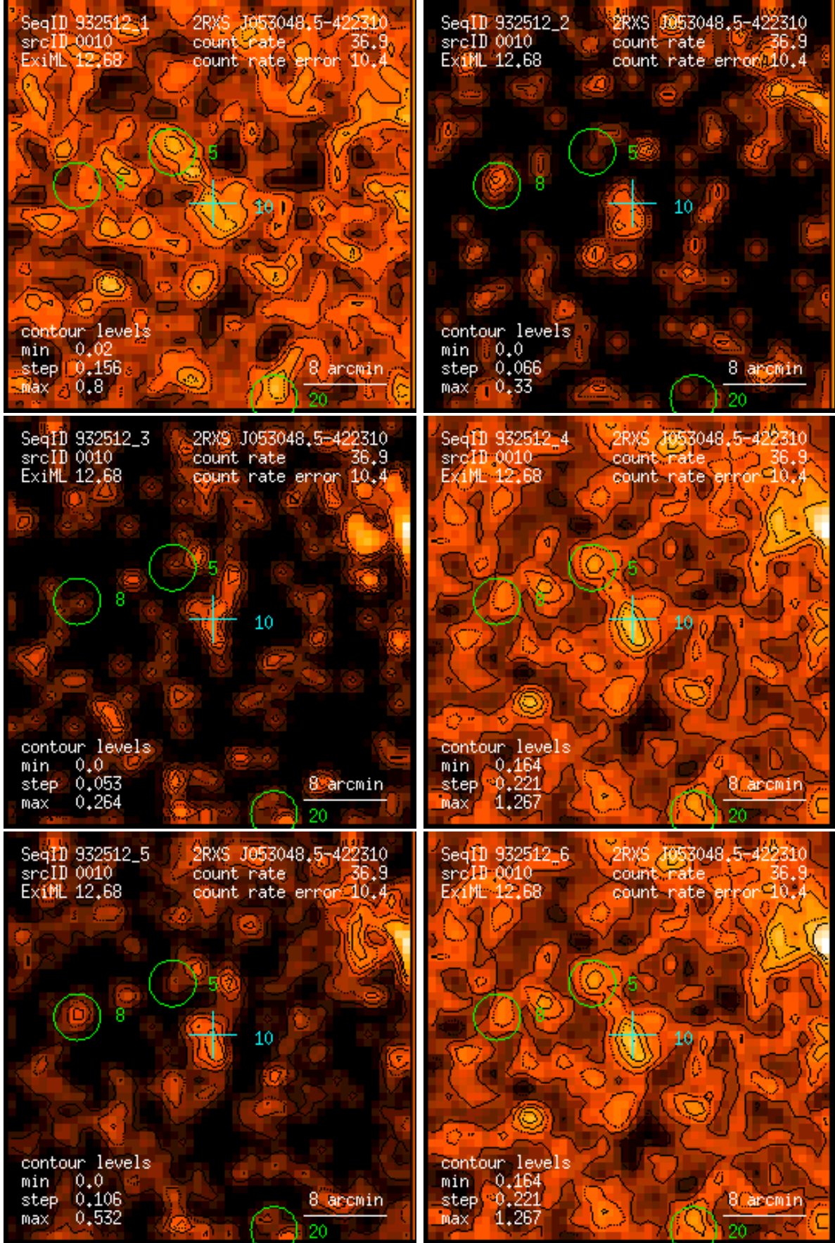
Figure 10: RASS 932512: detection 0010: band rate images, Gaussian filter: (1) PSPC channels 11 – 41, (2) 52 – 90, (3) 91 – 201, (4) 11 – 235, (5) 52 – 201, (6) 11 – 201. Broad band rates in counts/ks. Band rate contour levels in counts/ks/arcmin 2 .
