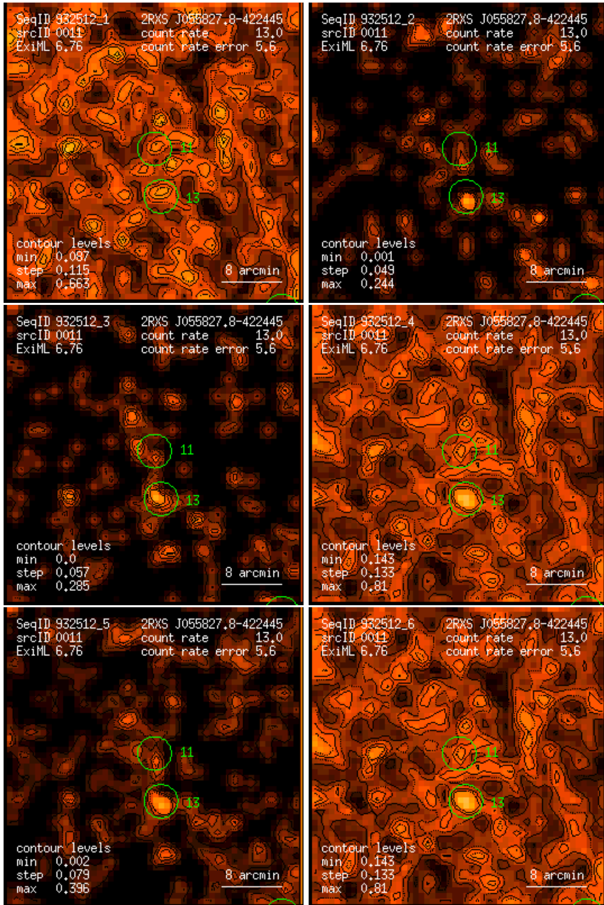
Figure 11: RASS 932512: detection 0011: band rate images, Gaussian filter: (1) PSPC channels 11 – 41, (2) 52 – 90, (3) 91 – 201, (4) 11 – 235, (5) 52 – 201, (6) 11 – 201. Broad band rates in counts/ks. Band rate contour levels in counts/ks/arcmin 2 .
