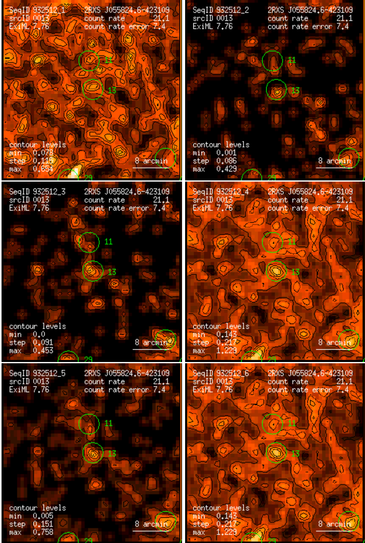
Figure 13: RASS 932512: detection 0013: band rate images, Gaussian filter: (1) PSPC channels 11 – 41, (2) 52 – 90, (3) 91 – 201, (4) 11 – 235, (5) 52 – 201, (6) 11 – 201. Broad band rates in counts/ks. Band rate contour levels in counts/ks/arcmin 2 .
