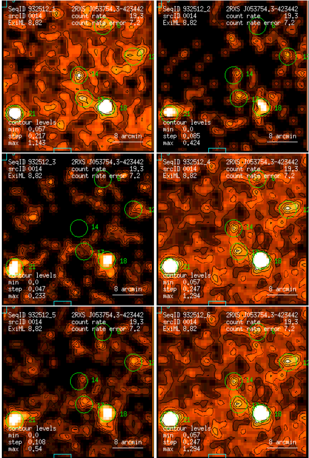
Figure 14: RASS 932512: detection 0014: band rate images, Gaussian filter: (1) PSPC channels 11 – 41, (2) 52 – 90, (3) 91 – 201, (4) 11 – 235, (5) 52 – 201, (6) 11 – 201. Broad band rates in counts/ks. Band rate contour levels in counts/ks/arcmin 2 .
