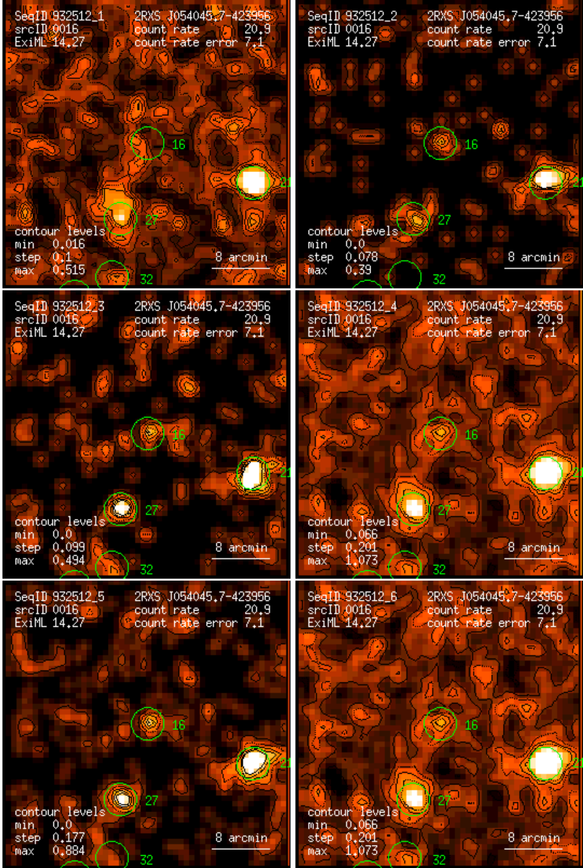
Figure 16: RASS 932512: detection 0016: band rate images, Gaussian filter: (1) PSPC channels 11 – 41, (2) 52 – 90, (3) 91 – 201, (4) 11 – 235, (5) 52 – 201, (6) 11 – 201. Broad band rates in counts/ks. Band rate contour levels in counts/ks/arcmin 2 .
