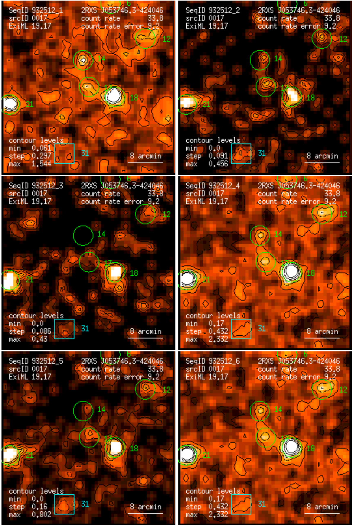
Figure 17: RASS 932512: detection 0017: band rate images, Gaussian filter: (1) PSPC channels 11 – 41, (2) 52 – 90, (3) 91 – 201, (4) 11 – 235, (5) 52 – 201, (6) 11 – 201. Broad band rates in counts/ks. Band rate contour levels in counts/ks/arcmin 2 .
