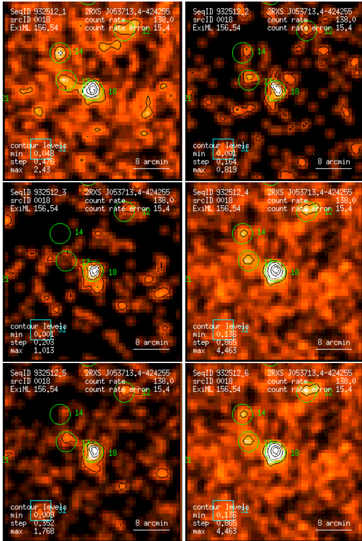
Figure 18: RASS 932512: detection 0018: band rate images, Gaussian filter: (1) PSPC channels 11 – 41, (2) 52 – 90, (3) 91 – 201, (4) 11 – 235, (5) 52 – 201, (6) 11 – 201. Broad band rates in counts/ks. Band rate contour levels in counts/ks/arcmin 2 .
