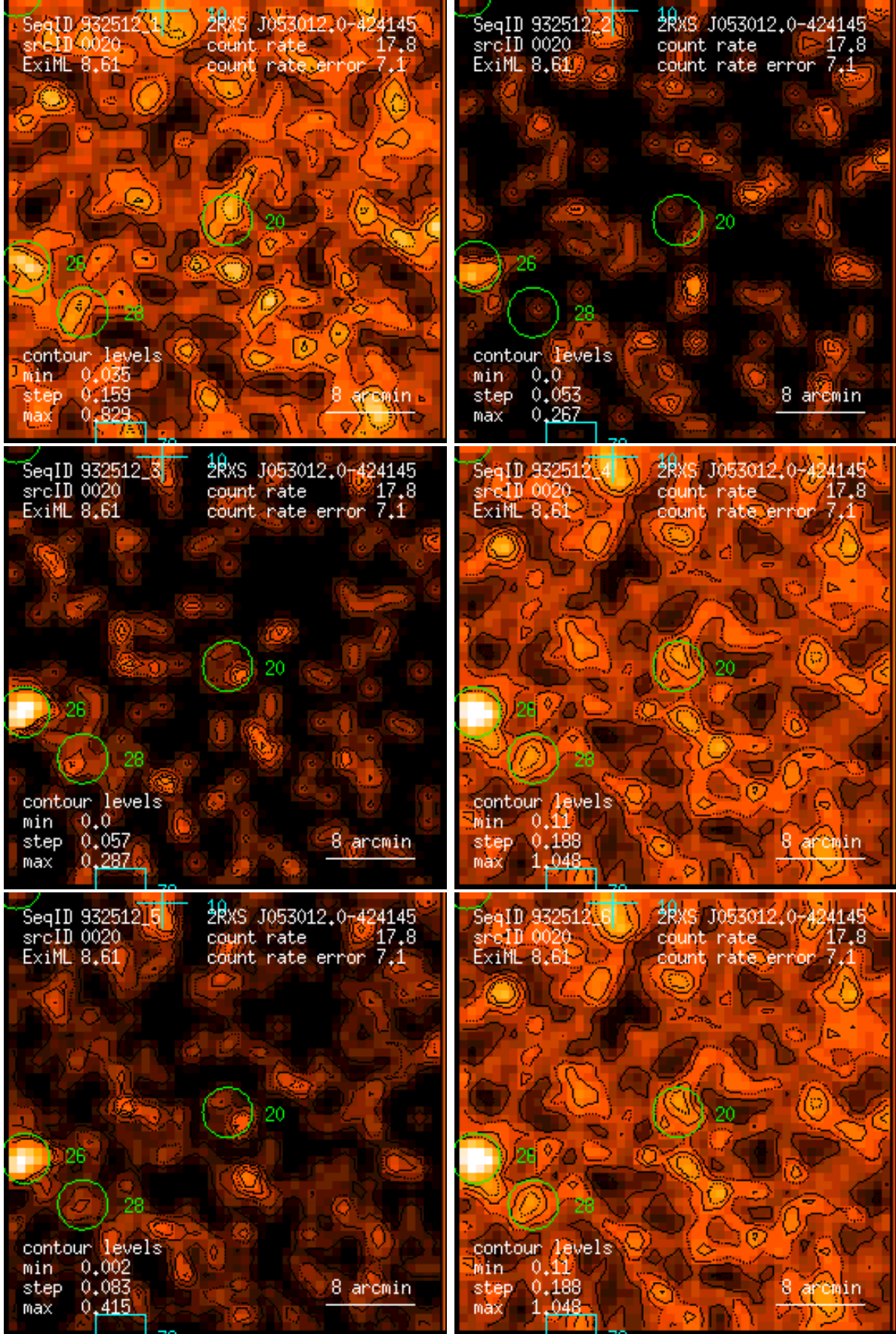
Figure 20: RASS 932512: detection 0020: band rate images, Gaussian filter: (1) PSPC channels 11 – 41, (2) 52 – 90, (3) 91 – 201, (4) 11 – 235, (5) 52 – 201, (6) 11 – 201. Broad band rates in counts/ks. Band rate contour levels in counts/ks/arcmin 2 .
