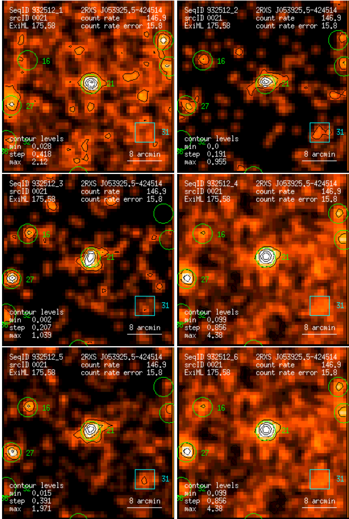
Figure 21: RASS 932512: detection 0021: band rate images, Gaussian filter: (1) PSPC channels 11 – 41, (2) 52 – 90, (3) 91 – 201, (4) 11 – 235, (5) 52 – 201, (6) 11 – 201. Broad band rates in counts/ks. Band rate contour levels in counts/ks/arcmin 2 .
