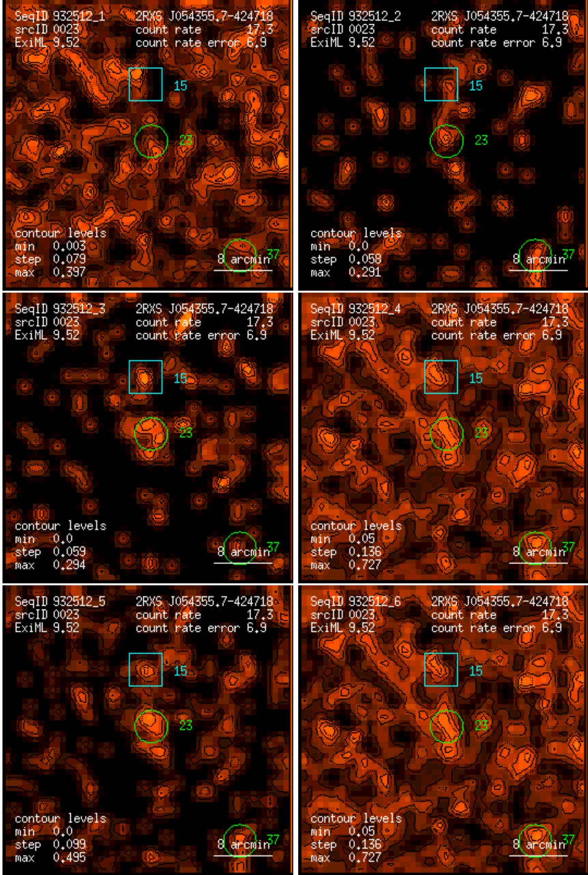
Figure 23: RASS 932512: detection 0023: band rate images, Gaussian filter: (1) PSPC channels 11 – 41, (2) 52 – 90, (3) 91 – 201, (4) 11 – 235, (5) 52 – 201, (6) 11 – 201. Broad band rates in counts/ks. Band rate contour levels in counts/ks/arcmin 2 .
