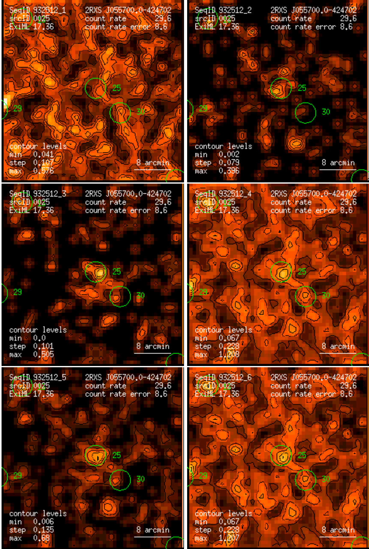
Figure 25: RASS 932512: detection 0025: band rate images, Gaussian filter: (1) PSPC channels 11 – 41, (2) 52 – 90, (3) 91 – 201, (4) 11 – 235, (5) 52 – 201, (6) 11 – 201. Broad band rates in counts/ks. Band rate contour levels in counts/ks/arcmin 2 .
