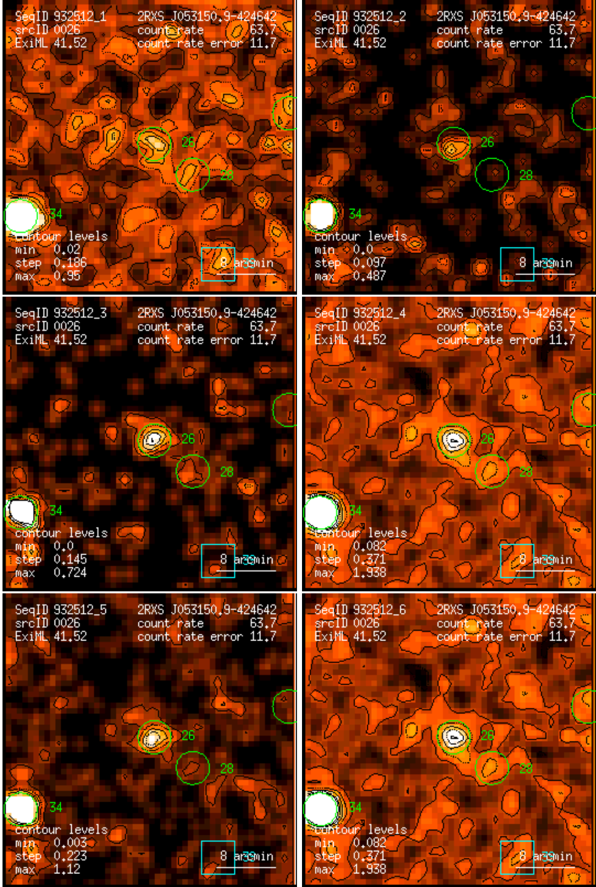
Figure 26: RASS 932512: detection 0026: band rate images, Gaussian filter: (1) PSPC channels 11 – 41, (2) 52 – 90, (3) 91 – 201, (4) 11 – 235, (5) 52 – 201, (6) 11 – 201. Broad band rates in counts/ks. Band rate contour levels in counts/ks/arcmin 2 .
