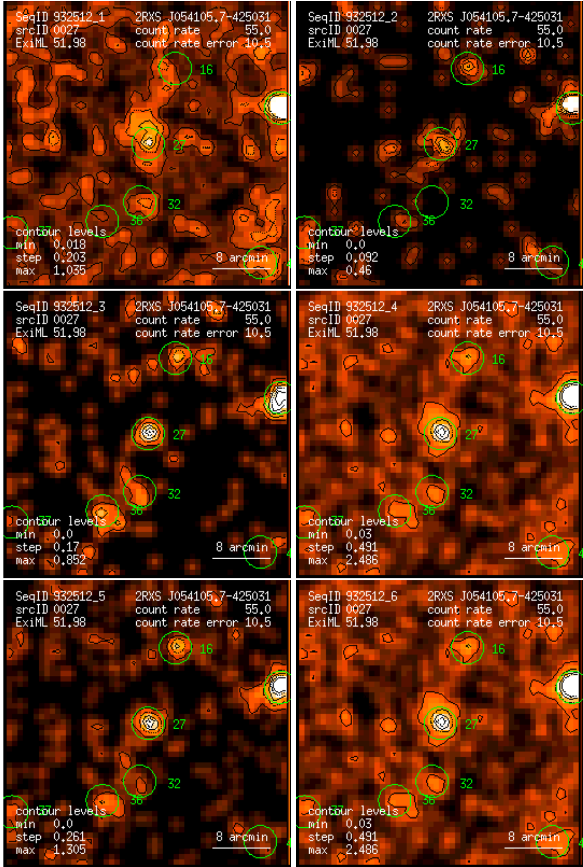
Figure 27: RASS 932512: detection 0027: band rate images, Gaussian filter: (1) PSPC channels 11 – 41, (2) 52 – 90, (3) 91 – 201, (4) 11 – 235, (5) 52 – 201, (6) 11 – 201. Broad band rates in counts/ks. Band rate contour levels in counts/ks/arcmin 2 .
