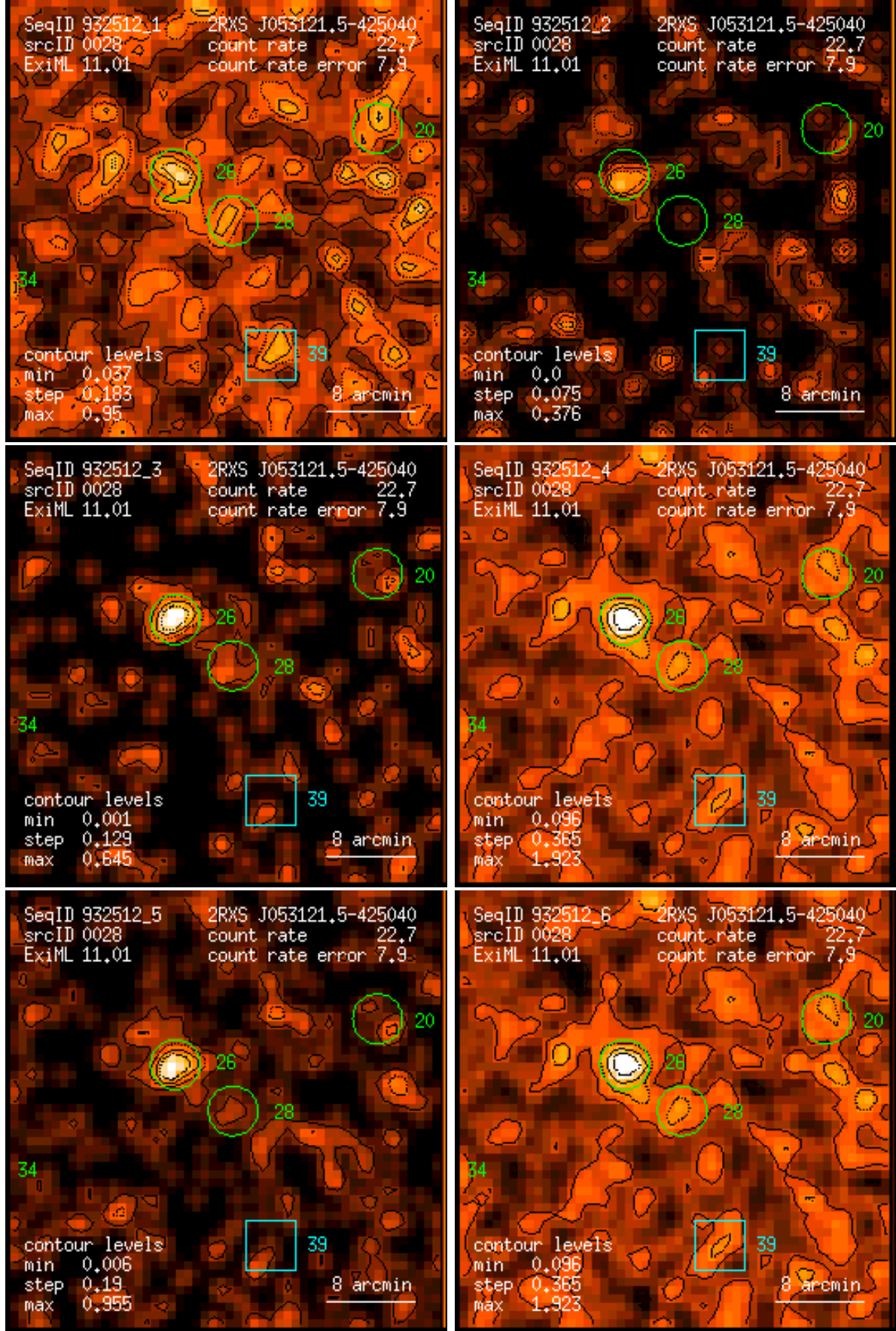
Figure 28: RASS 932512: detection 0028: band rate images, Gaussian filter: (1) PSPC channels 11 – 41, (2) 52 – 90, (3) 91 – 201, (4) 11 – 235, (5) 52 – 201, (6) 11 – 201. Broad band rates in counts/ks. Band rate contour levels in counts/ks/arcmin 2 .
