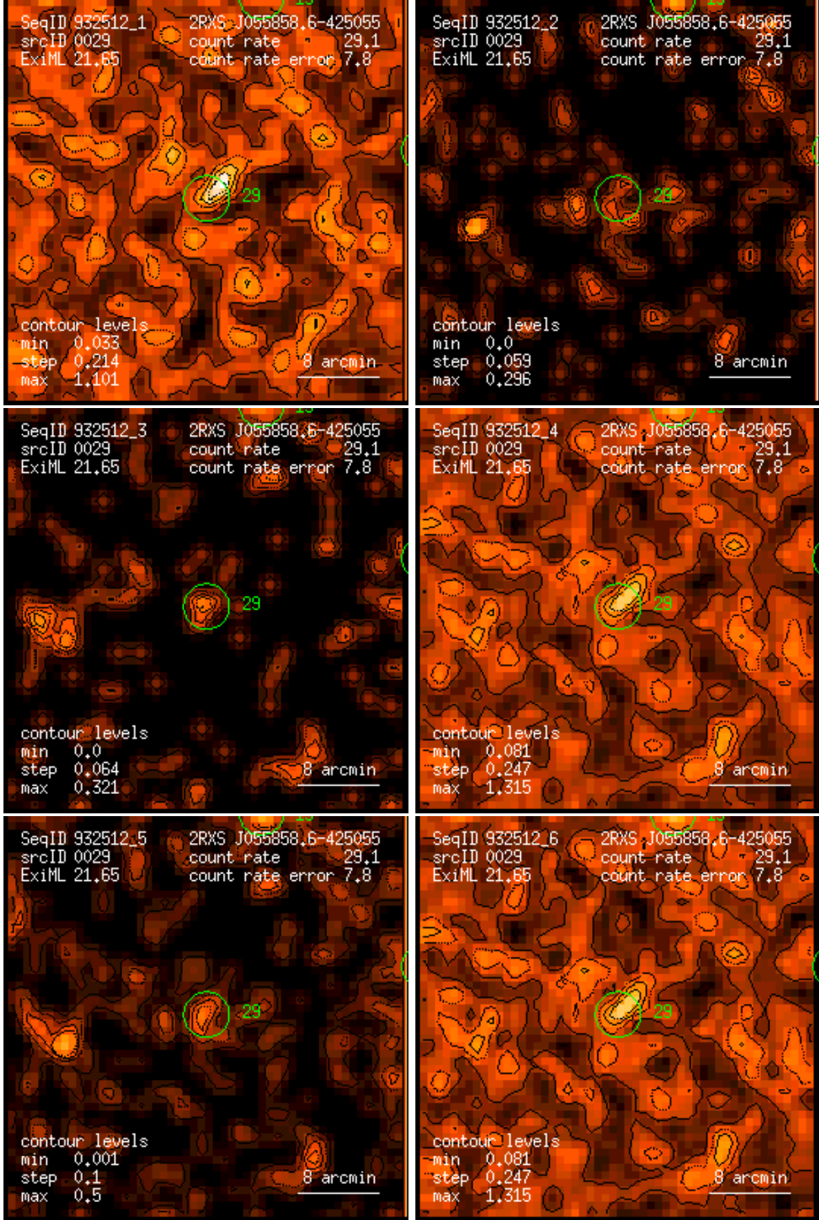
Figure 29: RASS 932512: detection 0029: band rate images, Gaussian filter: (1) PSPC channels 11 – 41, (2) 52 – 90, (3) 91 – 201, (4) 11 – 235, (5) 52 – 201, (6) 11 – 201. Broad band rates in counts/ks. Band rate contour levels in counts/ks/arcmin 2 .
