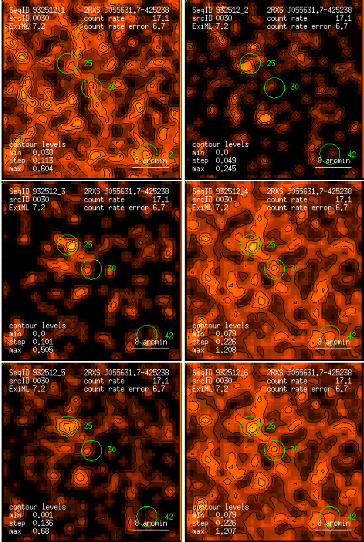
Figure 30: RASS 932512: detection 0030: band rate images, Gaussian filter: (1) PSPC channels 11 – 41, (2) 52 – 90, (3) 91 – 201, (4) 11 – 235, (5) 52 – 201, (6) 11 – 201. Broad band rates in counts/ks. Band rate contour levels in counts/ks/arcmin 2 .
