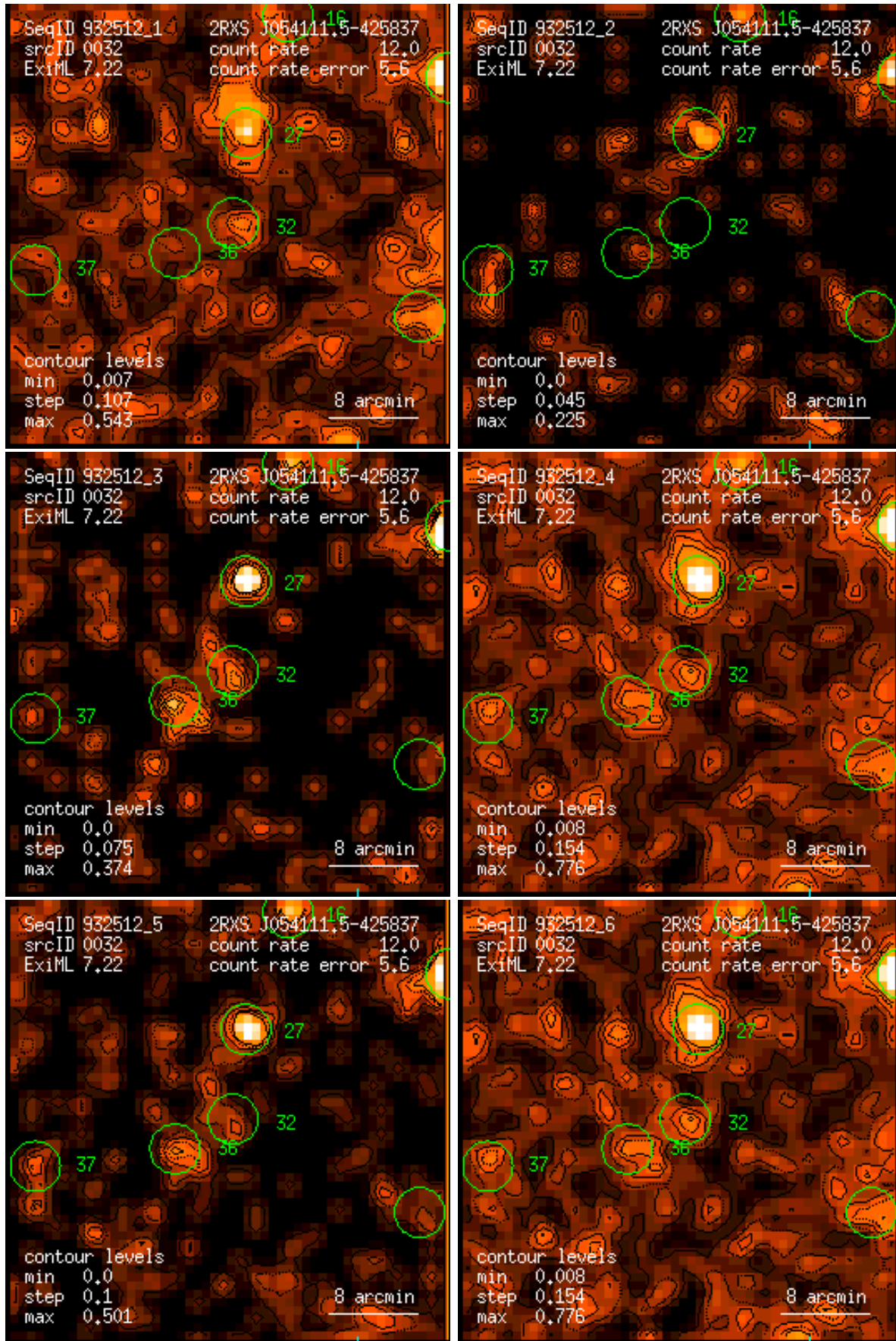
Figure 32: RASS 932512: detection 0032: band rate images, Gaussian filter: (1) PSPC channels 11 – 41, (2) 52 – 90, (3) 91 – 201, (4) 11 – 235, (5) 52 – 201, (6) 11 – 201. Broad band rates in counts/ks. Band rate contour levels in counts/ks/arcmin 2 .
