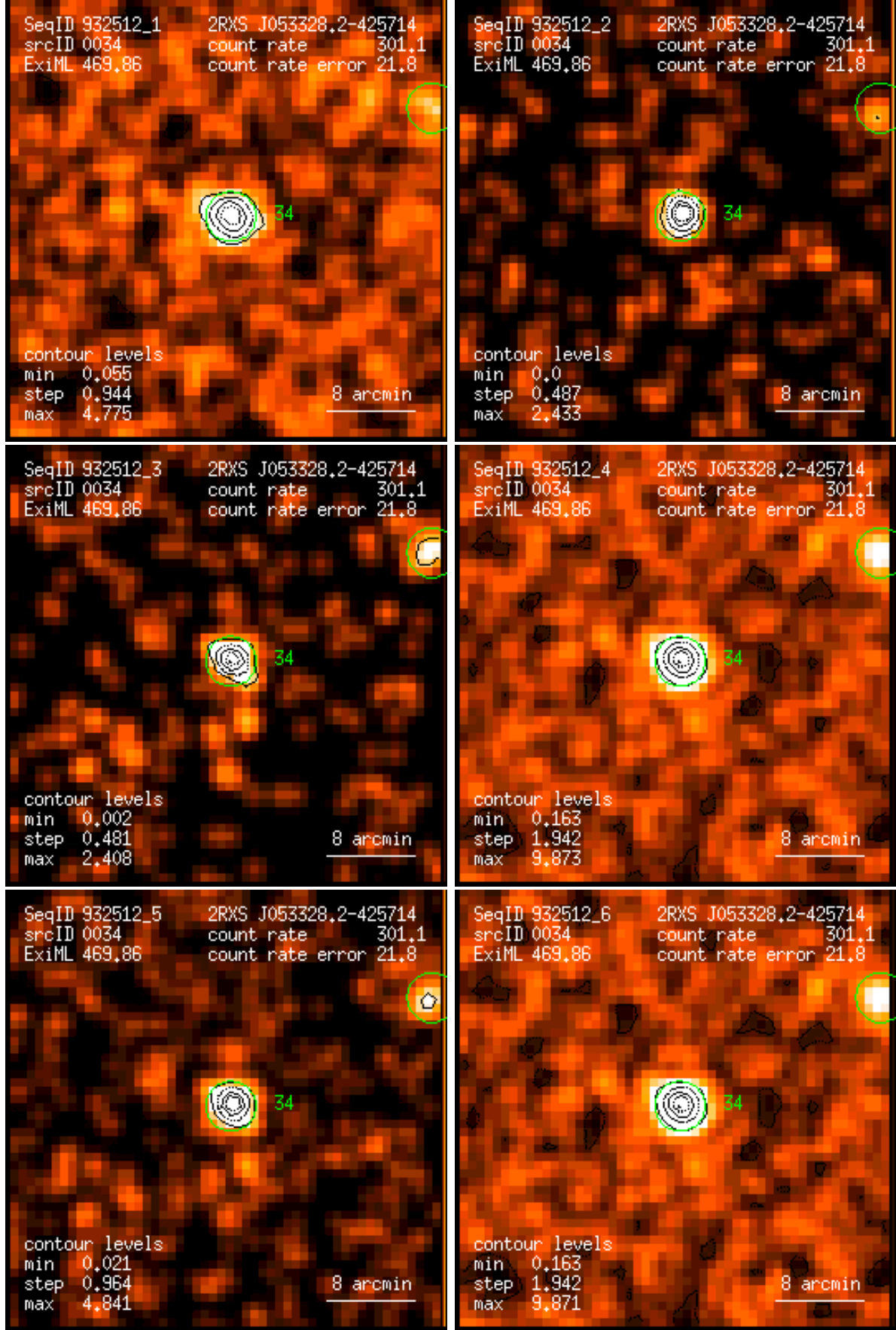
Figure 34: RASS 932512: detection 0034: band rate images, Gaussian filter: (1) PSPC channels 11 – 41, (2) 52 – 90, (3) 91 – 201, (4) 11 – 235, (5) 52 – 201, (6) 11 – 201. Broad band rates in counts/ks. Band rate contour levels in counts/ks/arcmin 2 .
