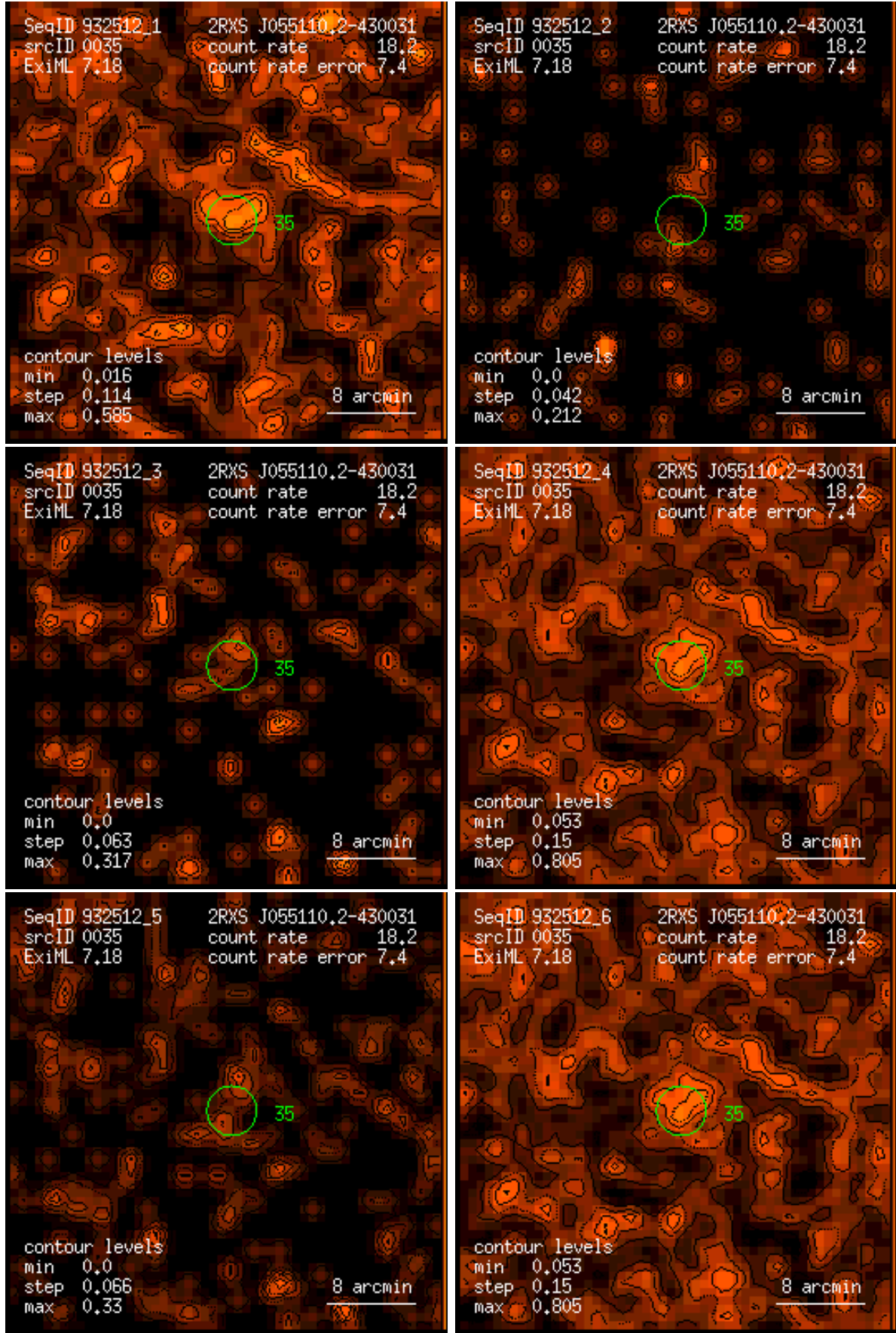
Figure 35: RASS 932512: detection 0035: band rate images, Gaussian filter: (1) PSPC channels 11 – 41, (2) 52 – 90, (3) 91 – 201, (4) 11 – 235, (5) 52 – 201, (6) 11 – 201. Broad band rates in counts/ks. Band rate contour levels in counts/ks/arcmin 2 .
