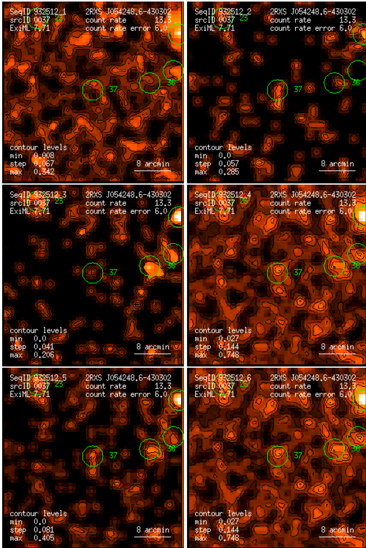
Figure 37: RASS 932512: detection 0037: band rate images, Gaussian filter: (1) PSPC channels 11 – 41, (2) 52 – 90, (3) 91 – 201, (4) 11 – 235, (5) 52 – 201, (6) 11 – 201. Broad band rates in counts/ks. Band rate contour levels in counts/ks/arcmin 2 .
