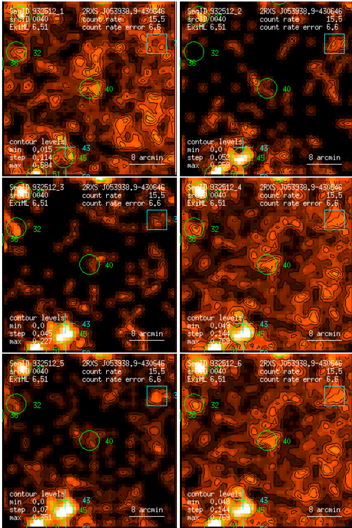
Figure 40: RASS 932512: detection 0040: band rate images, Gaussian filter: (1) PSPC channels 11 – 41, (2) 52 – 90, (3) 91 – 201, (4) 11 – 235, (5) 52 – 201, (6) 11 – 201. Broad band rates in counts/ks. Band rate contour levels in counts/ks/arcmin 2 .
