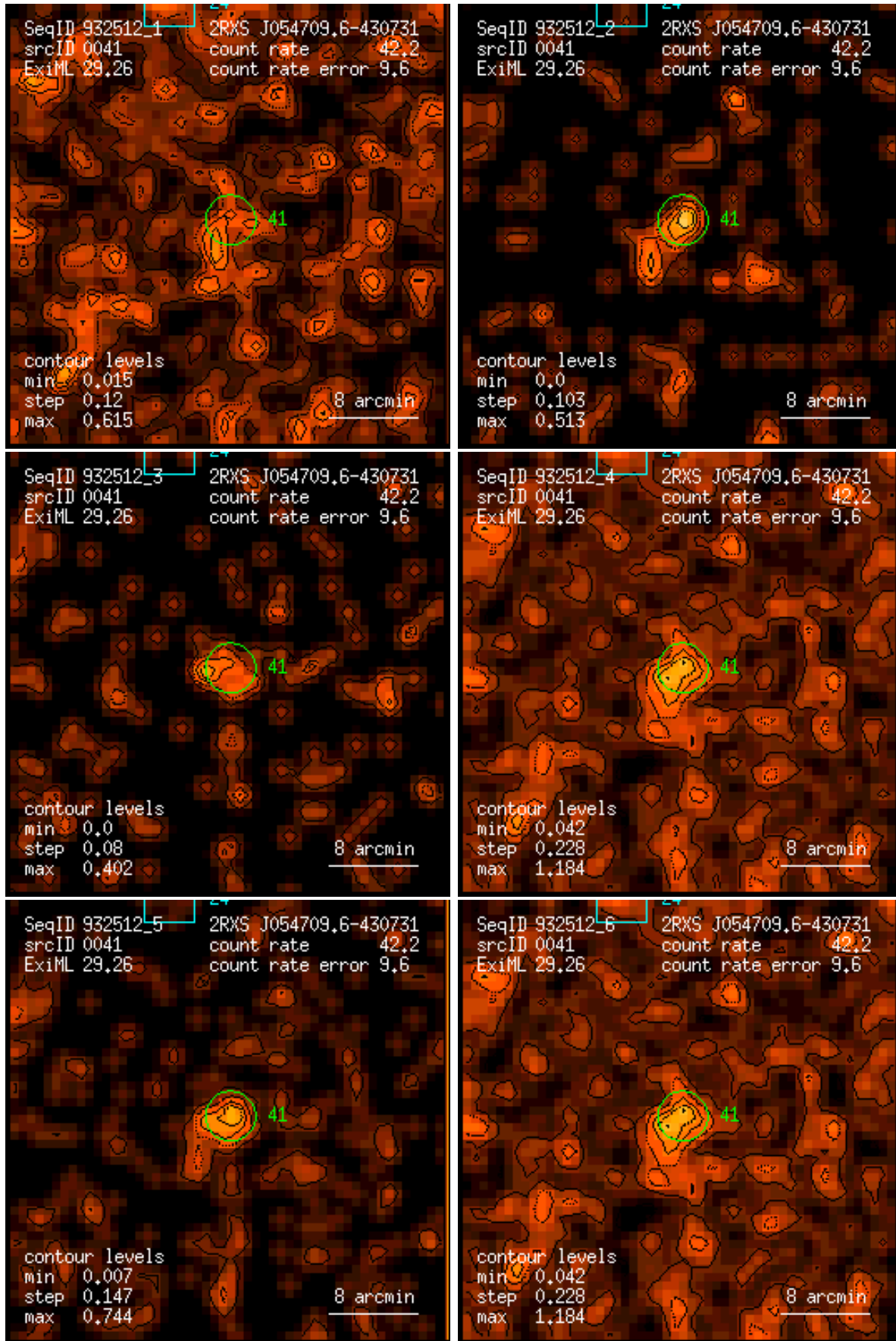
Figure 41: RASS 932512: detection 0041: band rate images, Gaussian filter: (1) PSPC channels 11 – 41, (2) 52 – 90, (3) 91 – 201, (4) 11 – 235, (5) 52 – 201, (6) 11 – 201. Broad band rates in counts/ks. Band rate contour levels in counts/ks/arcmin 2 .
