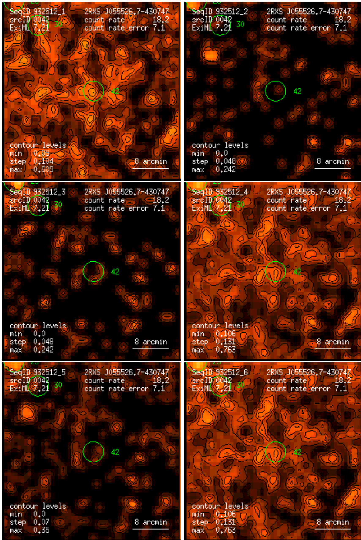
Figure 42: RASS 932512: detection 0042: band rate images, Gaussian filter: (1) PSPC channels 11 – 41, (2) 52 – 90, (3) 91 – 201, (4) 11 – 235, (5) 52 – 201, (6) 11 – 201. Broad band rates in counts/ks. Band rate contour levels in counts/ks/arcmin 2 .
